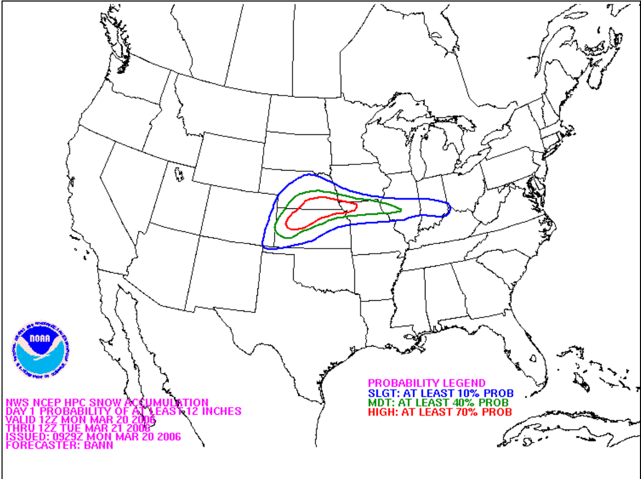
Figure 3. DIP12S - Day 1 Probability of Receiving at Least 12" Snow
