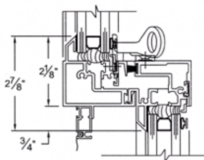
FIGURE 9 Section detail showing custom muntin simulating the meeting rails of a double hung window with upper and lower sash in two planes. (Courtesy of WINCO)
