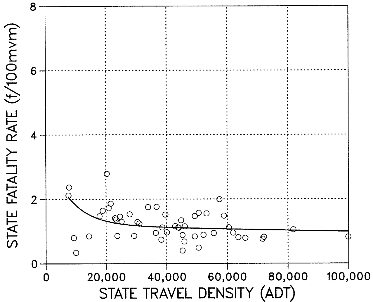
Fig. 7-C1c. PROVISIONAL RATE-DENSITY RELATIONSHIP (1981-84) URBAN INTERSTATE SYSTEM
