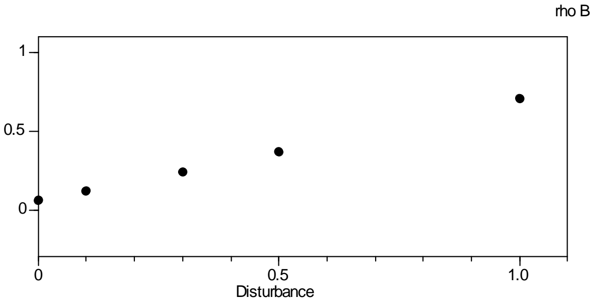
Figure 6. Relationship between rho (y-axis) and the level of bias introduced in the data (x-axis). The monotonically increasing relationship indicates that larger biases in the data do produce larger rho values.
