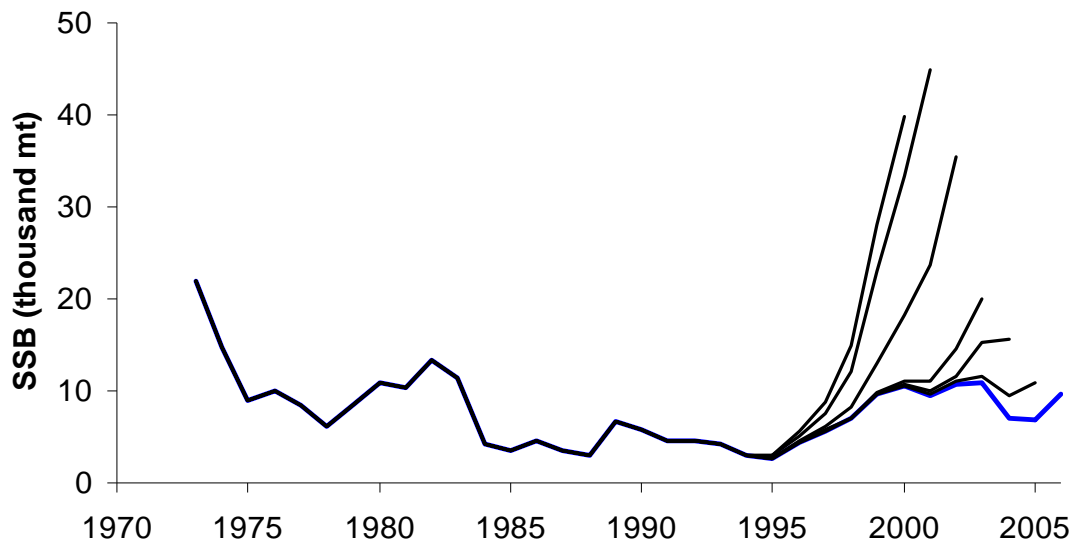
Figure 3. A strong retrospective pattern observed in the 2007 Georges Bank yellowtail flounder Base Case assessment.
