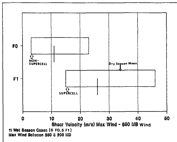
FIG. 10. Box and whisker diagram illustrating the range of shear velocities ( m s^{-1} ) between the maximum upper-tropospheric wind (350–200 mb) and 850-mb wind for six F0 and five F1 wet-season tornado cases (including two from Golden and Sabones 1991). Confirmed supercell and nonsupercell maximum shear values of the two Golden and Sabones (1991) cases are indicated by arrows. Mean shear of F0 and F1 cases indicated by vertical lines. Mean shear of dry-season proximity cases indicated by arrow.
