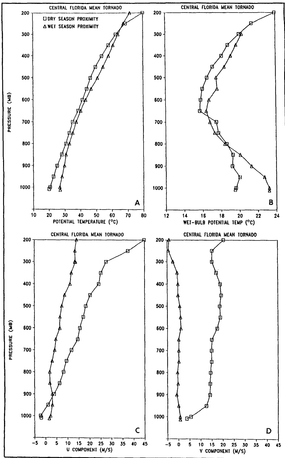
FIG. 6. Mean vertical profiles of \theta (a), \theta_w (b), U (c), and V (d) to 200 mb for mean dry- and wet-season tornado-proximity cases.
