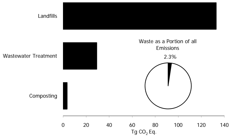
Figure 8-1: 2007 Waste Chapter Greenhouse Gas Sources
