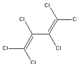
Hexachlorobutadiene
