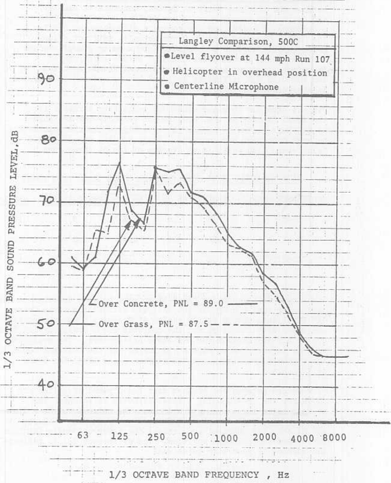
FIGURE 59 MICROPHONE REFLECTING SURFACE COMPARISON Helicopter Noise Measurement Program
