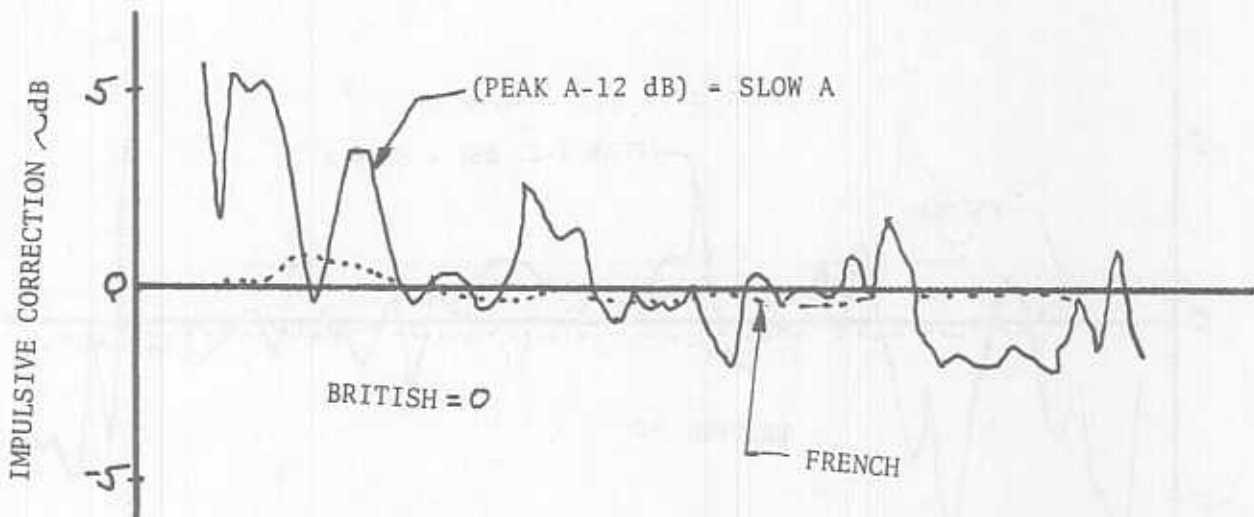
IMPULSIVE CORRECTIONS FOR 500C, 130mph
