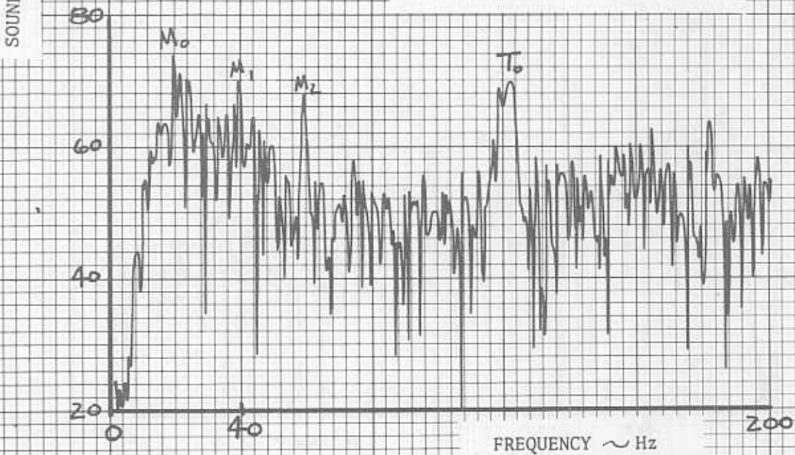
FIGURE 107 S-61(SH-3), RUN 32, CENTERLINE MICROPHONE
