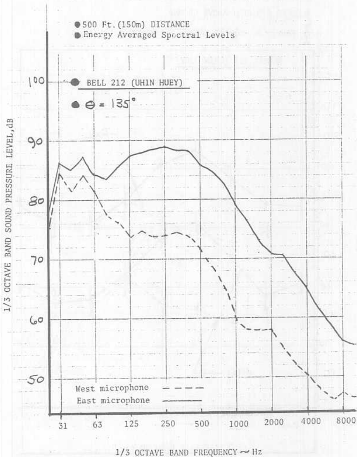
FIGURE 85. FIVE FOOT HOVER SPECTRA
