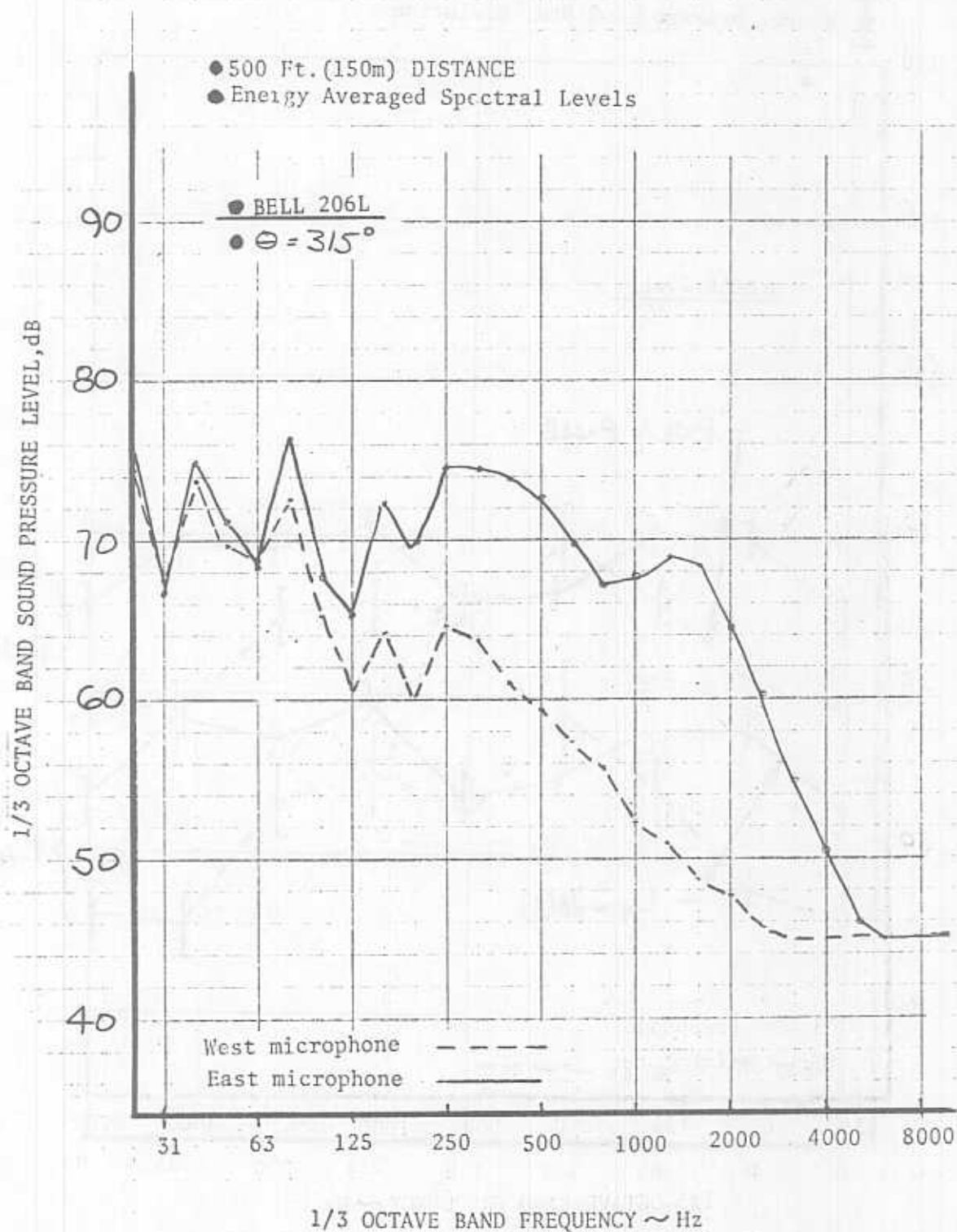
FIGURE 9/. FIVE FOOT HOVER SPECTRA
