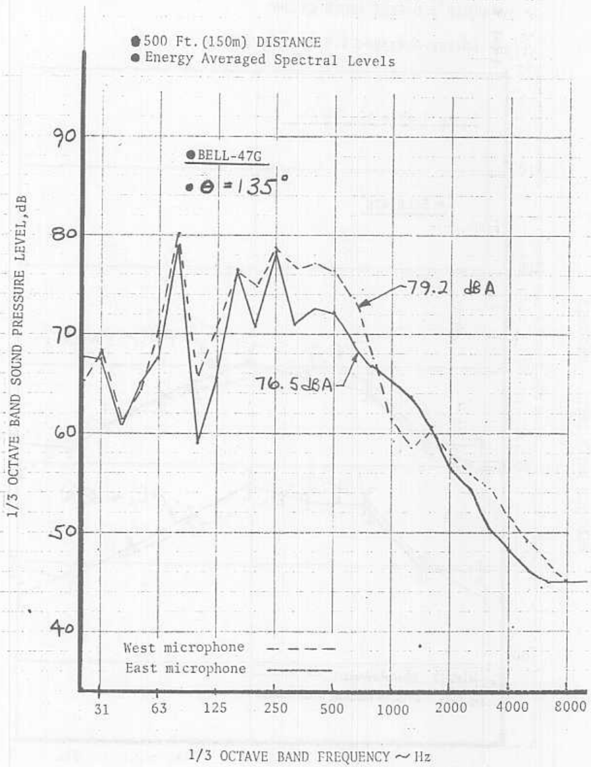
FIGURE 23. FIVE FOOT HOVER SPECTRA
