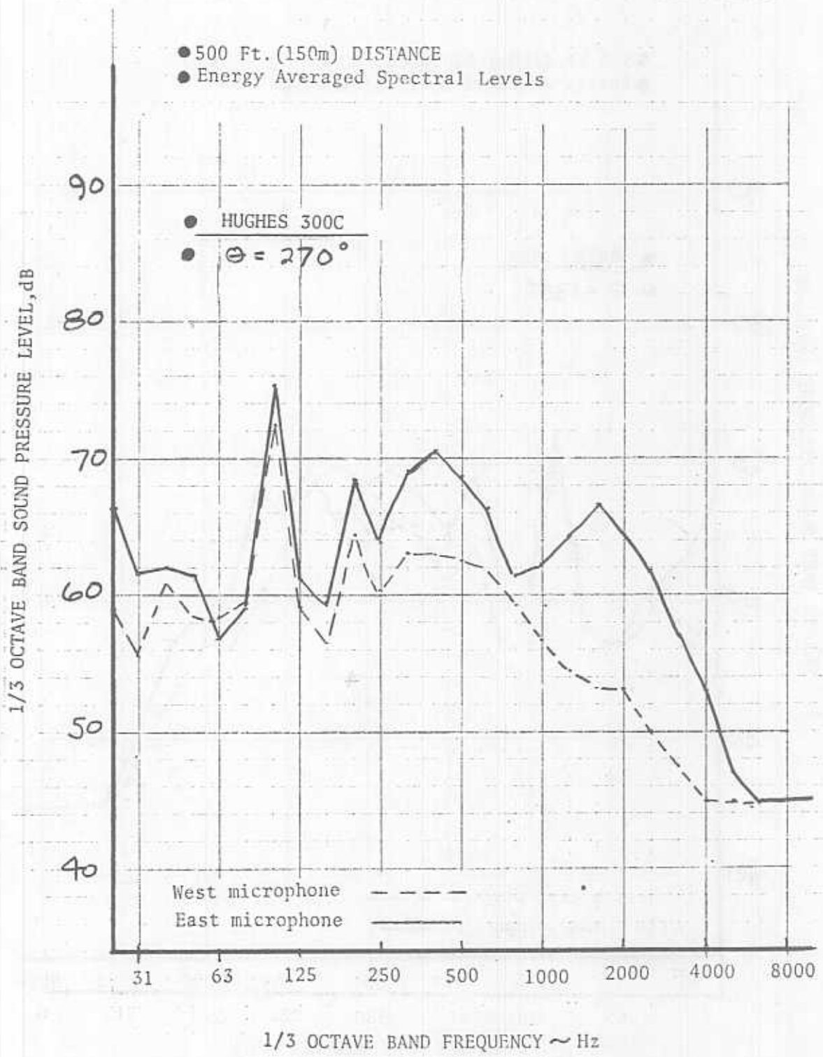
FIGURE 89. FIVE FOOT HOVER SPECTRA
