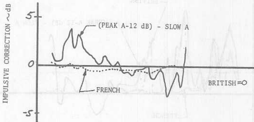
FIGURE 113 IMPULSIVE CORRECTIONS FOR BELL-47G, 75mph
