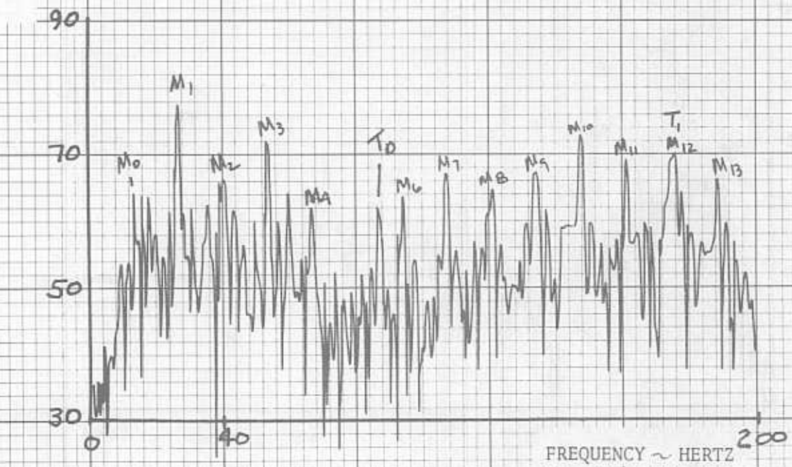
FIGURE 102, BELL 206L, RUN 59, CENTERLINE MICROPHONE
