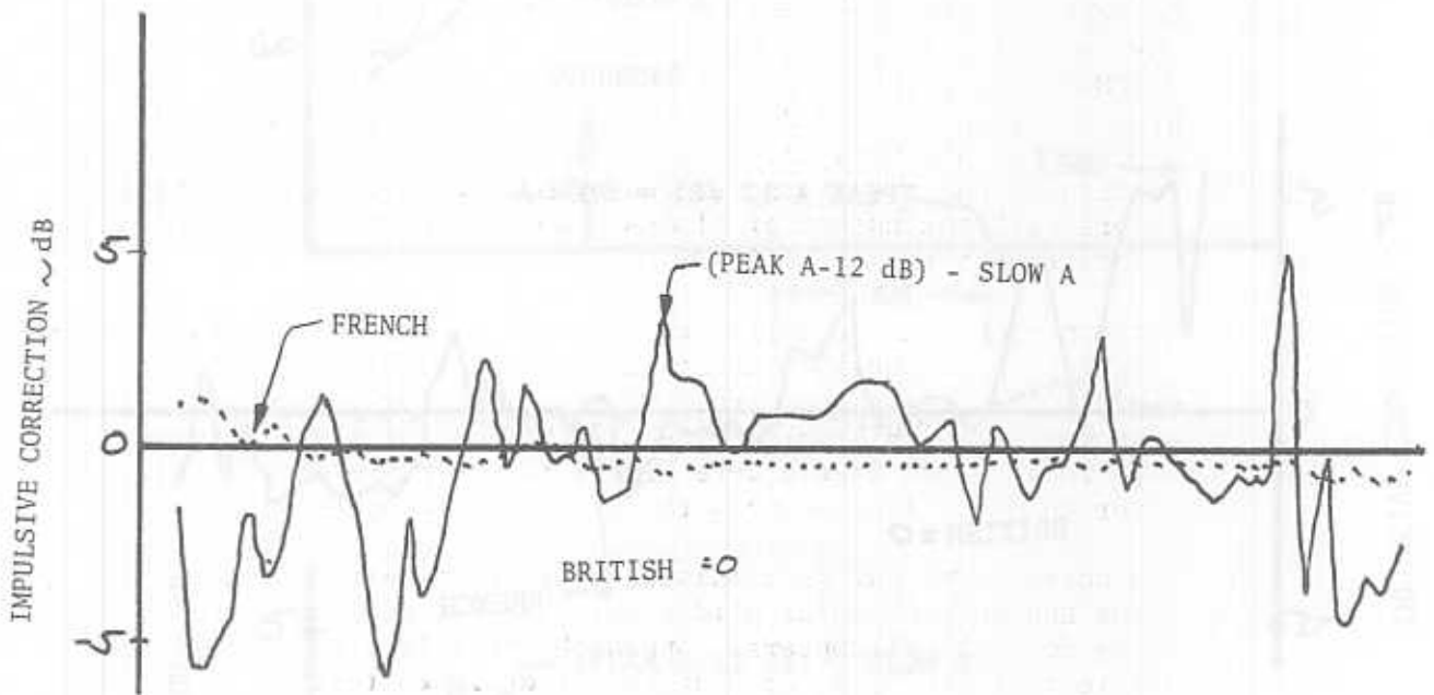
IMPULSIVE CORRECTIONS FOR 300C, 75mph
