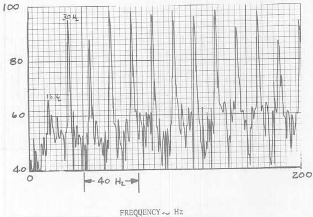
FIGURE 98 CH-47C, RUN 27, CENTERLINE MICROPHONE
