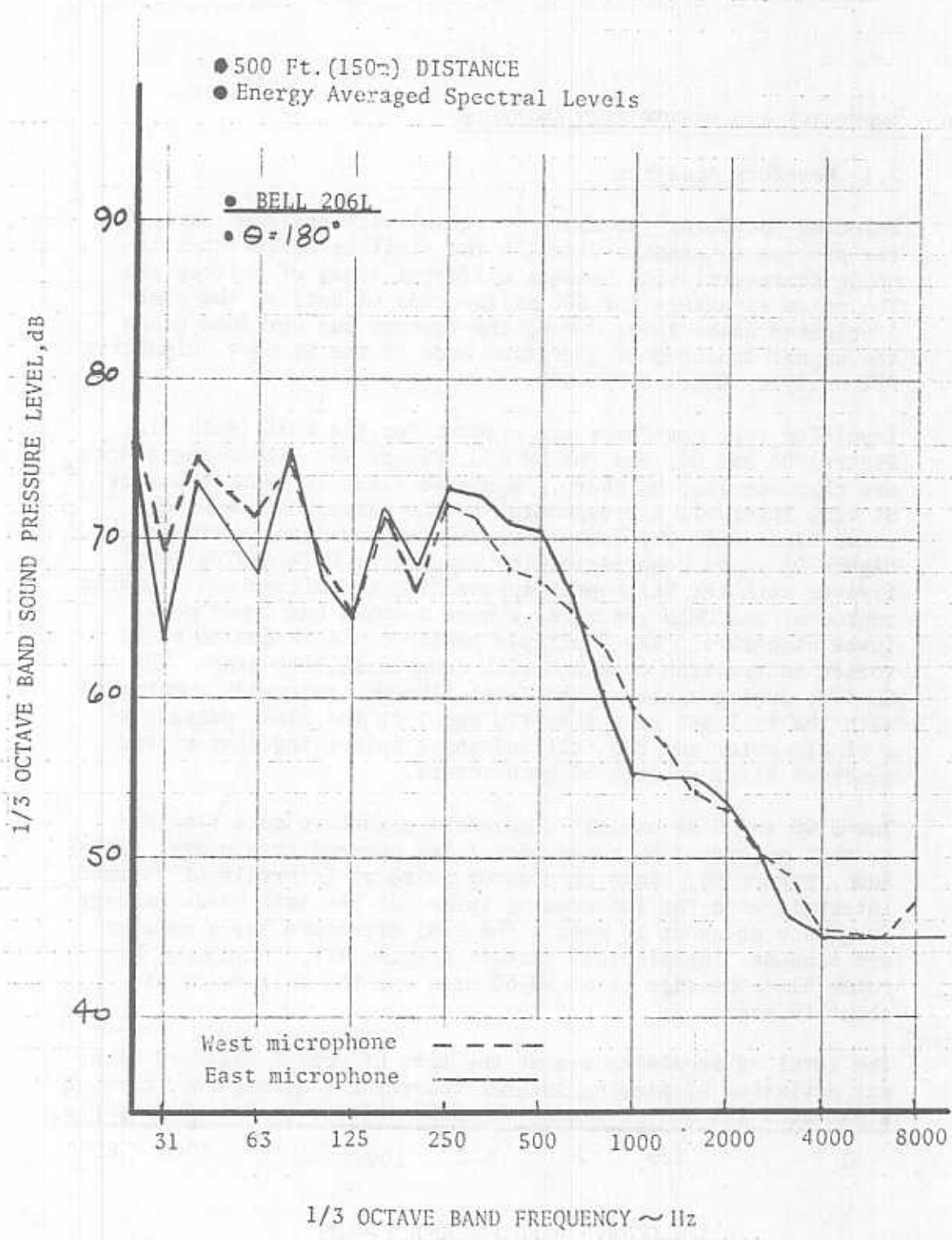
FIGURE 7a. FIVE FOOT HOVER SPECTRA
