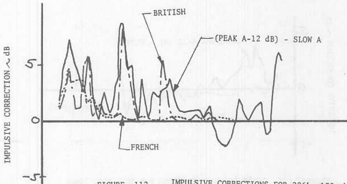
FIGURE 112 IMPULSIVE CORRECTIONS FOR 206L, 130mph
