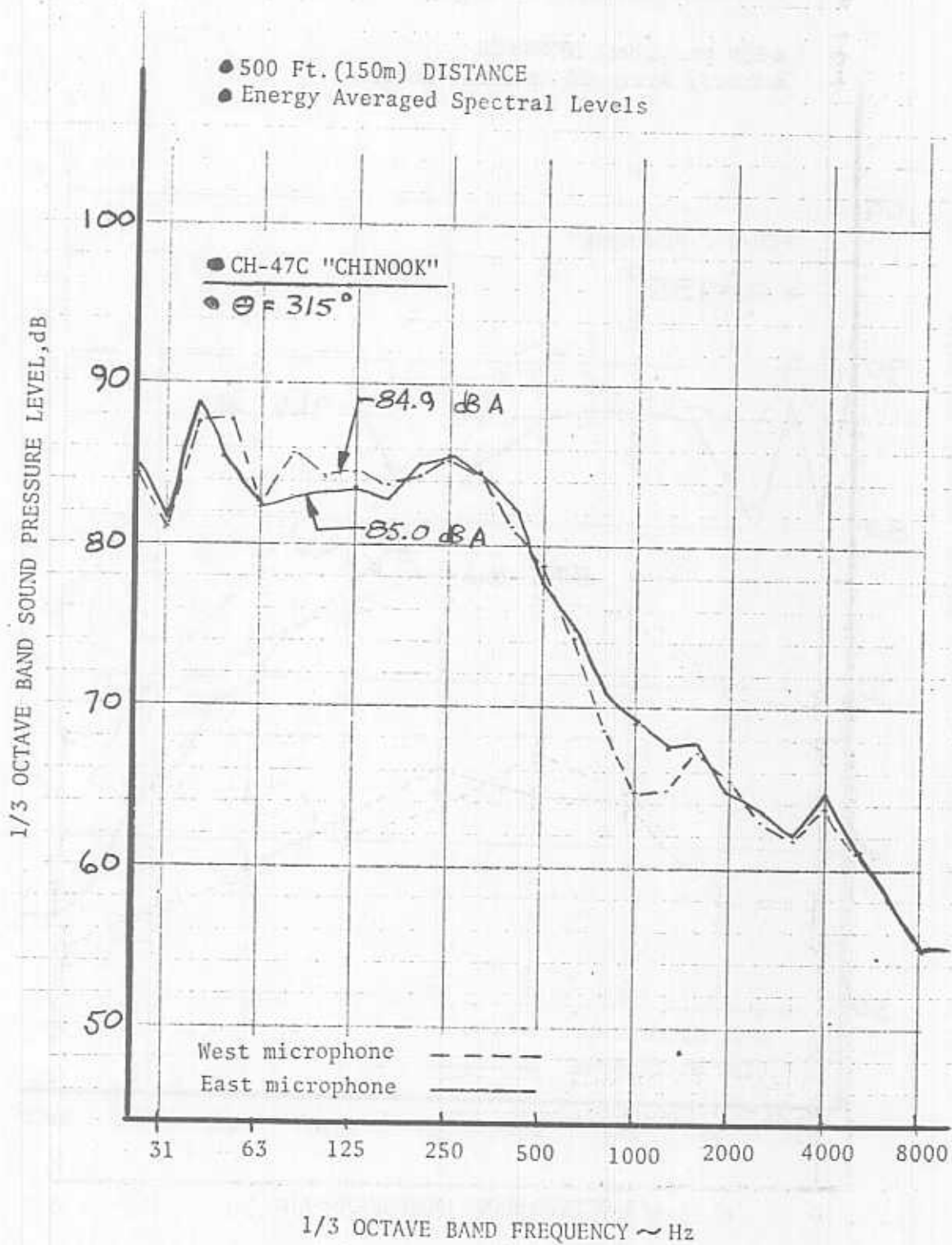
FIGURE 71. FIVE FOOT HOVER SPECTRA
