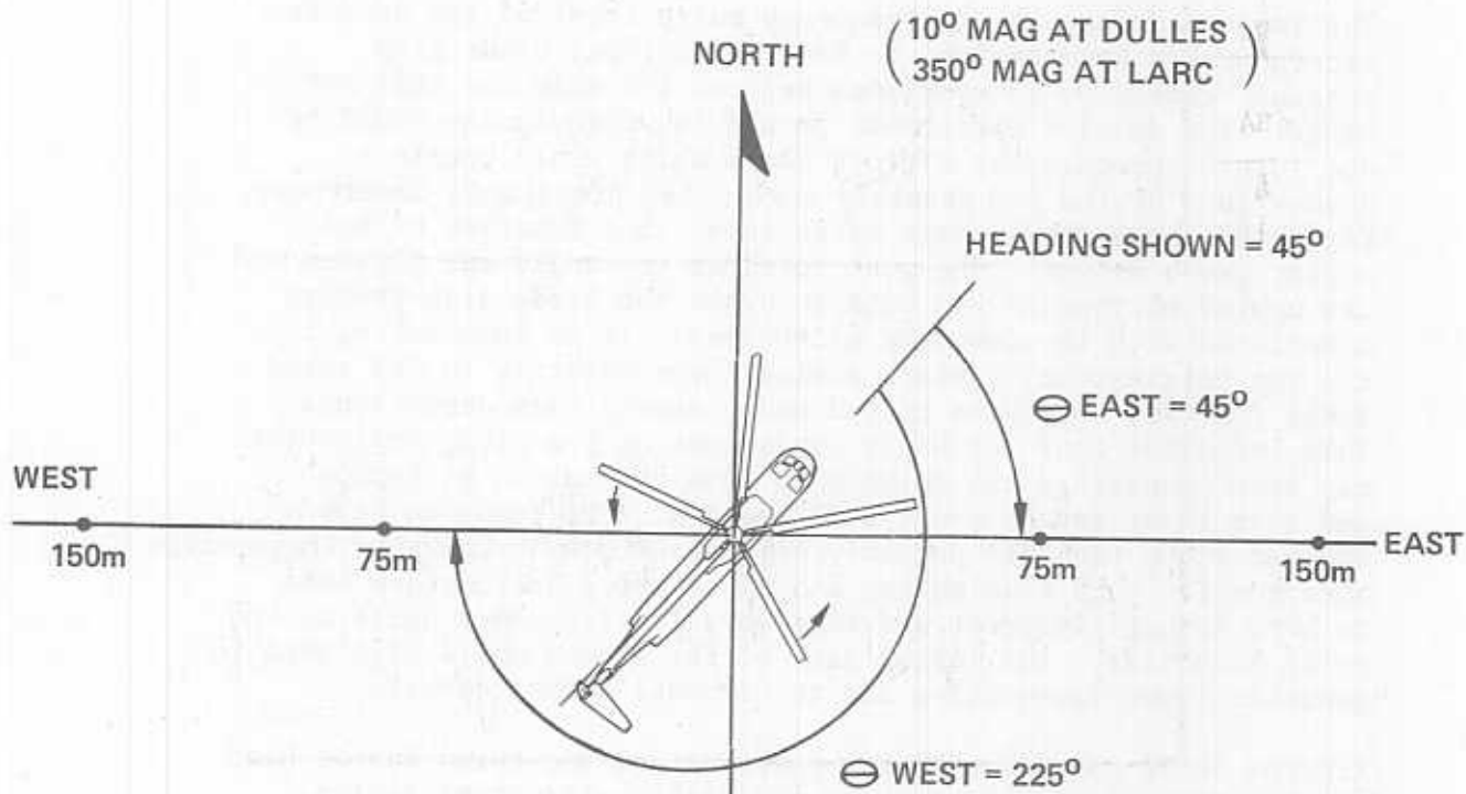
(a) PLAN VIEW OF TEST
