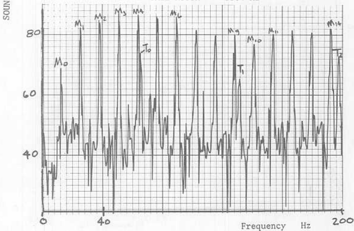
FIGURE 100 UHIN, RUN 37 WEST S.L. MICROPHONE FLYOVER LOCATION = 11 SEC BEFORE OVERHEAD
