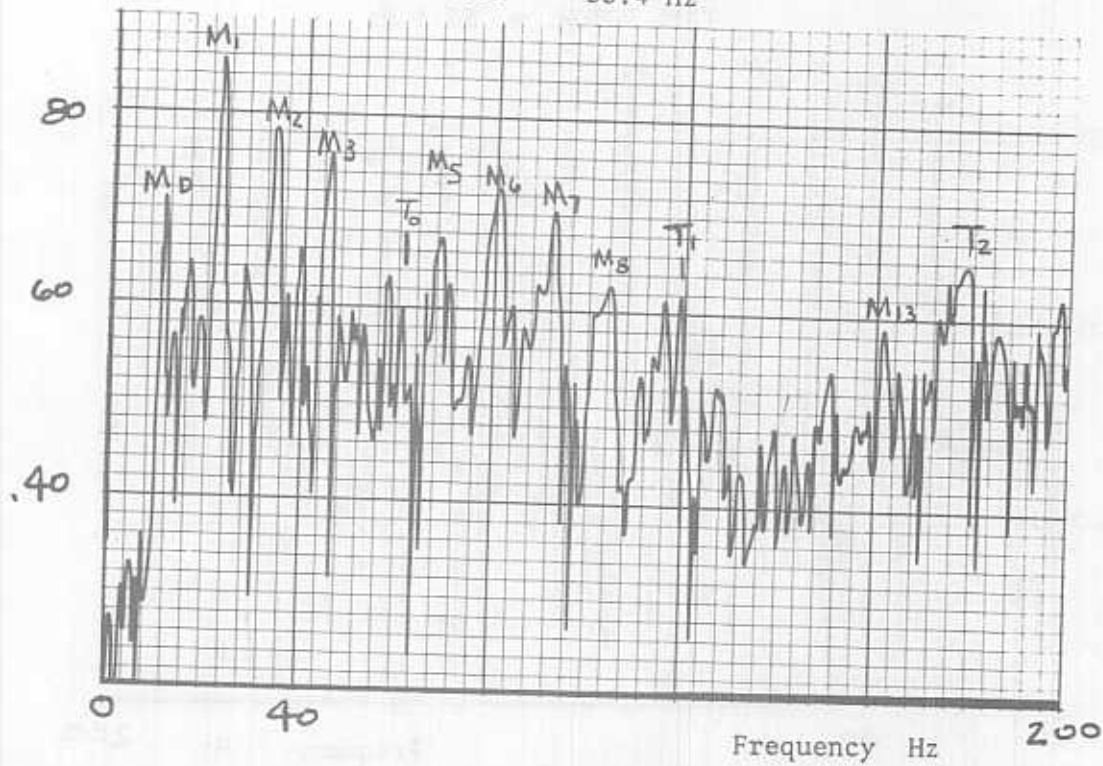
FIGURE 101 UHIN, RUN 37 WEST S.L. MICROPHONE FLYOVER LOCATION = OVERHEAD
