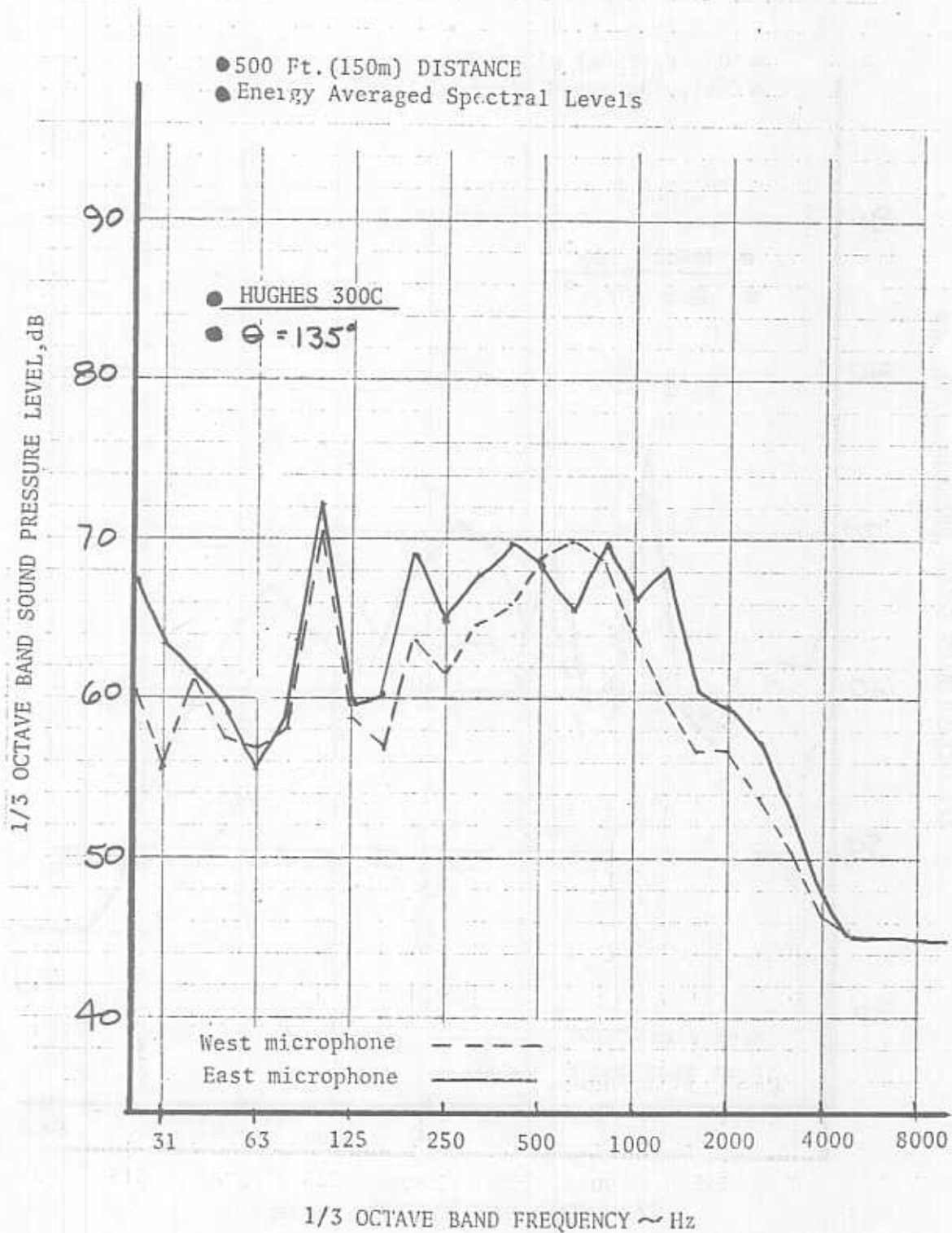
FIGURE 88. FIVE FOOT HOVER SPECTRA
