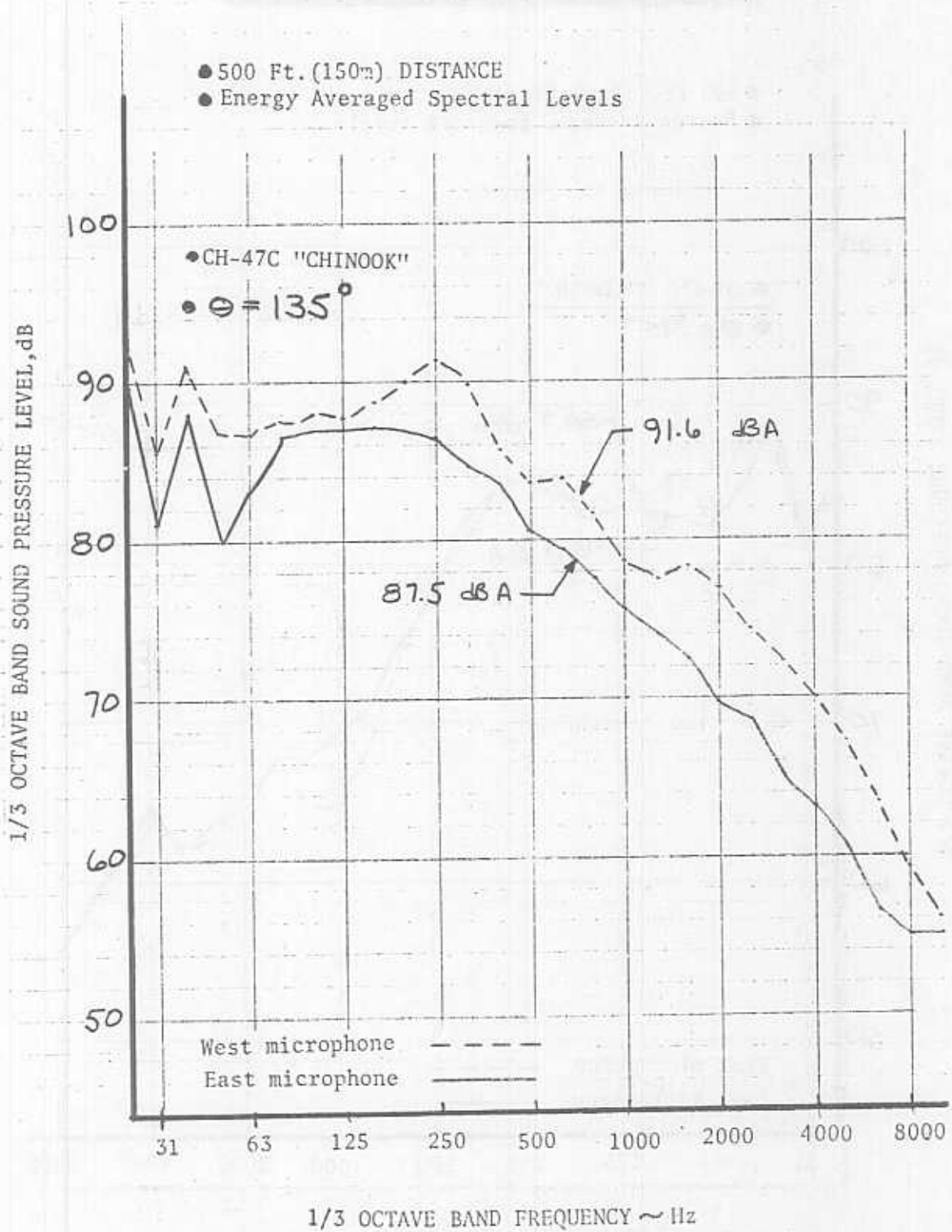
FIGURE 70. FIVE FOOT HOVER SPECTRA
