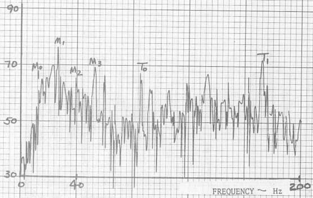
FIGURE 103, BELL 206L, RUN 59, CENTERLINE MICROPHONE
