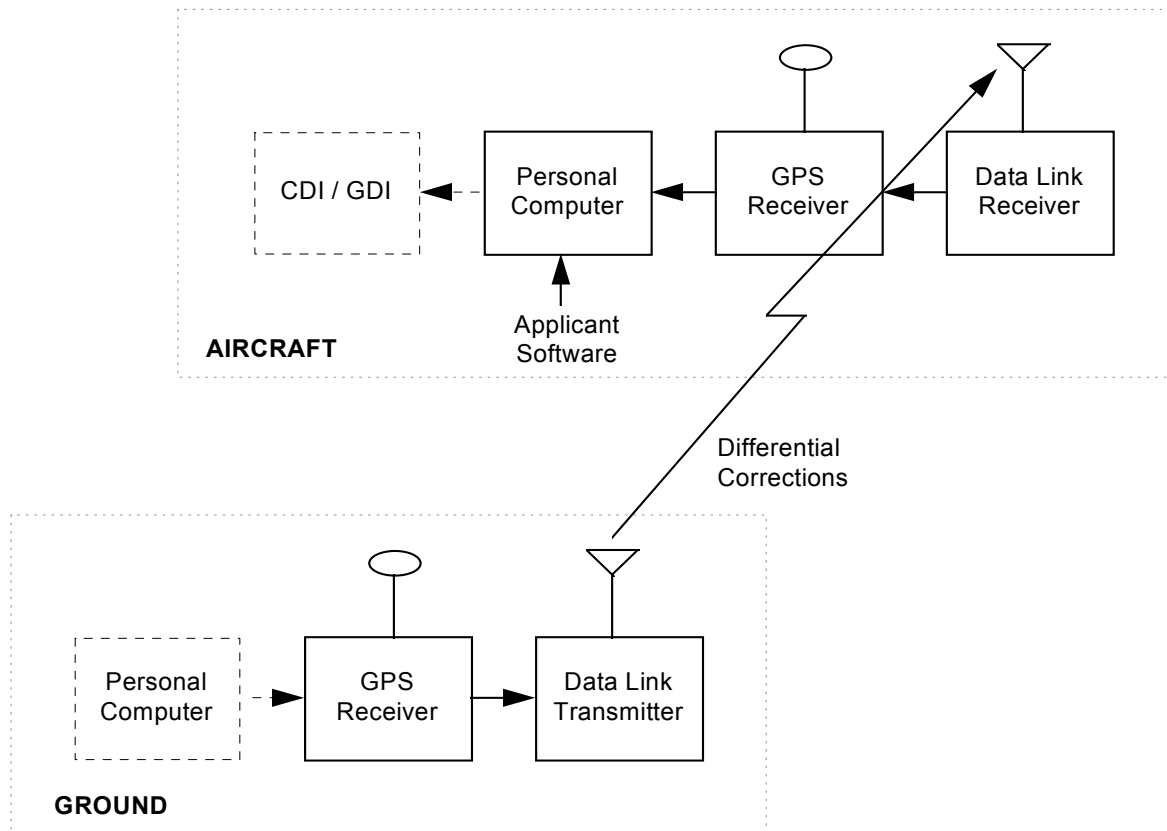
Figure 1: DGPS TSPI System Basic Architecture
