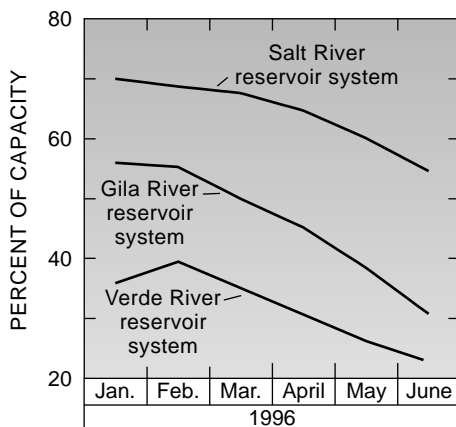
Figure 3. Amount of water available in central Arizona reservoirs since January, 1996; as a percentage of total storage capacity (Dallas Riegle, Senior Hydrologist, Salt River Project, written commun., 1996).
