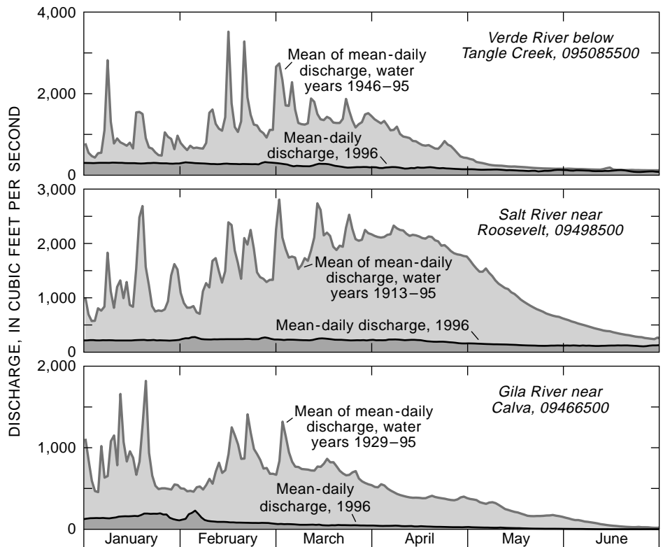
Figure 2. Mean-daily discharge for January 1 to June 30, 1996, and the mean of the mean-daily discharges for the period of record at Verde River below Tangle Creek, Salt River near Roosevelt, and Gila River near Calva (data for 1996 are provisional and are subject to revision).
