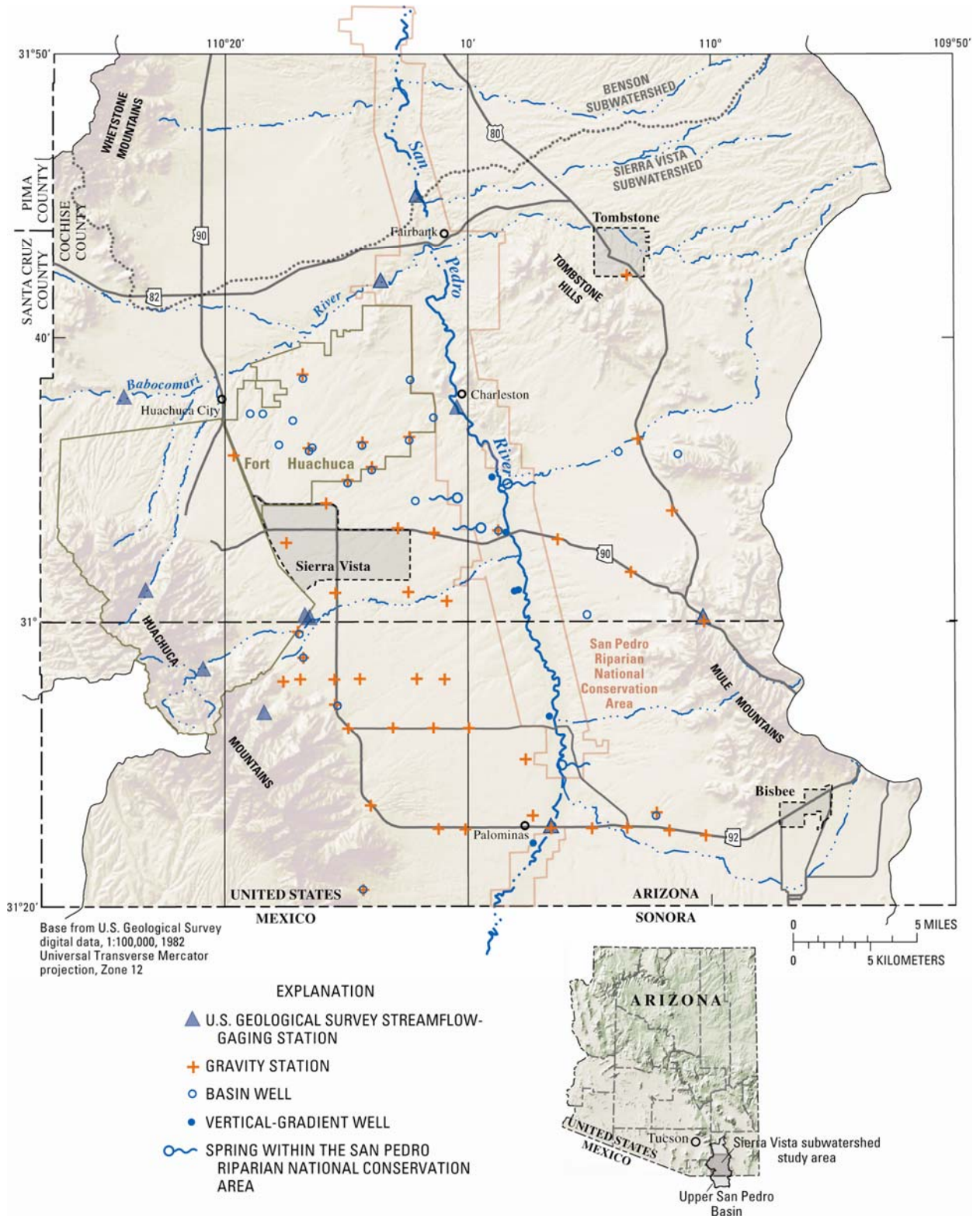
Figure 3. Locations of streamflow, ground-water level, spring, and microgravity monitoring locations in the Sierra Vista Subwatershed, Upper San Pedro Basin, Arizona.
