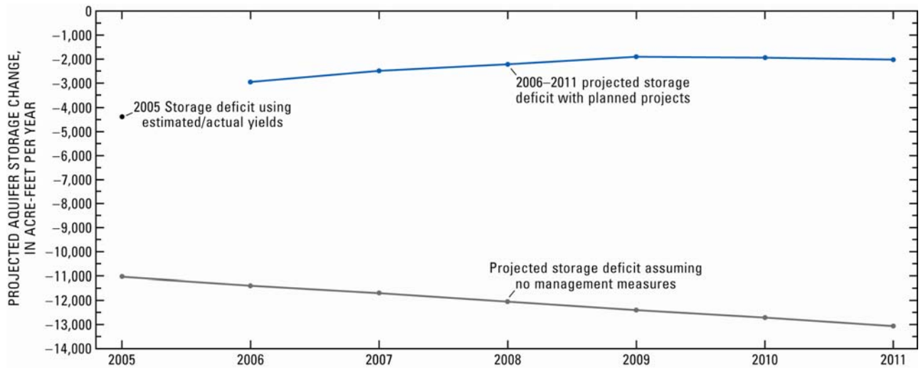
Figure 2. Effect of management measure yields (planned yields and estimates of actual yields) on annual aquifer storage change (calculated as the difference between projected annual aquifer-storage depletions if no management measures are taken and management-measure yields).
