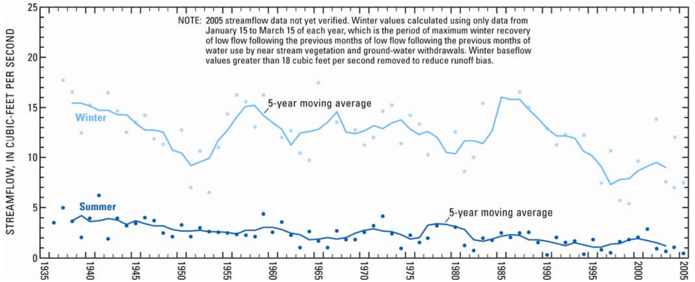
Figure 5. Seasonal 7-day low flow at the San Pedro River at Charleston streamflow-gaging station.
