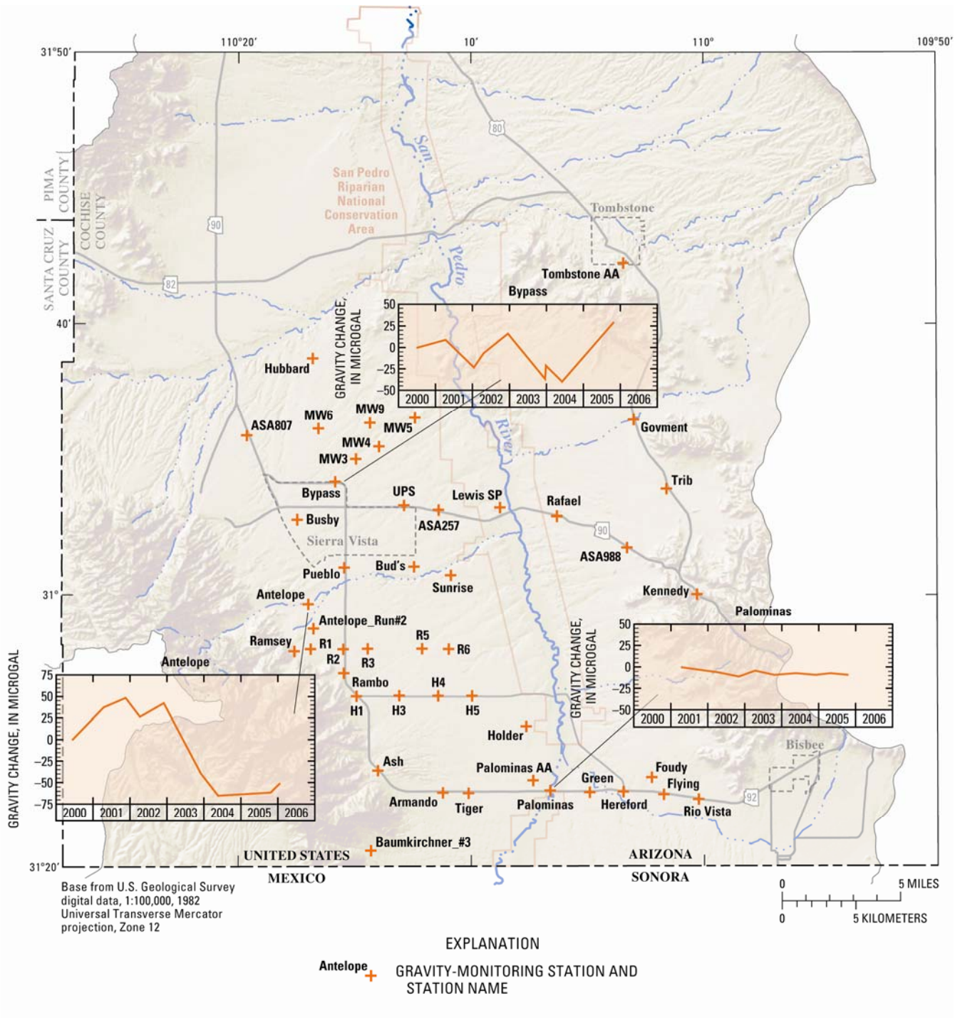
Figure 8. Microgravity monitoring locations and changes in gravity at selected locations, Sierra Vista Subwatershed, Upper San Pedro Basin, Arizona, 2000–2006.
