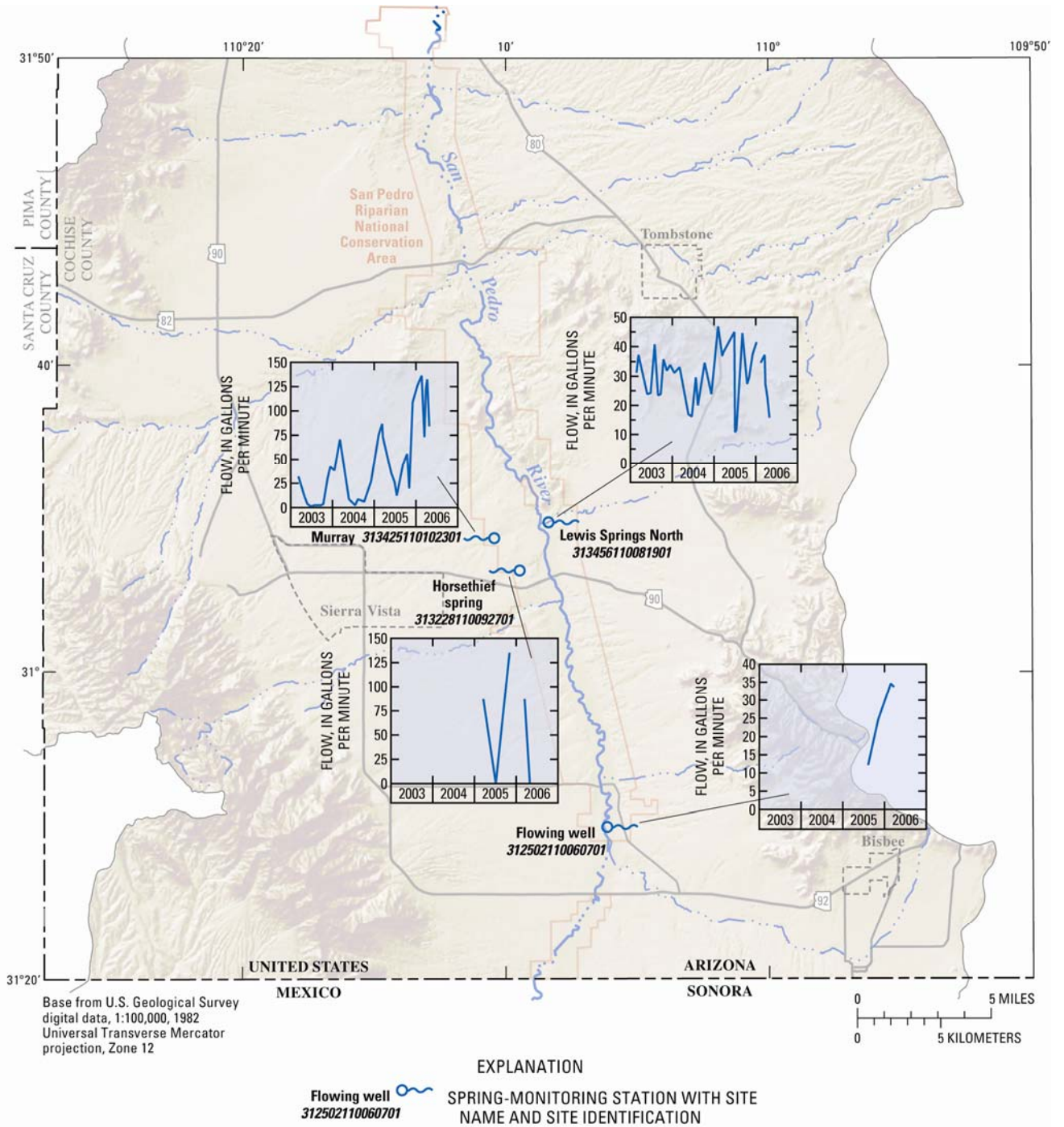
Figure 6. Measured flow at spring-monitoring locations, Sierra Vista Subwatershed, Upper San Pedro Basin, Arizona.
