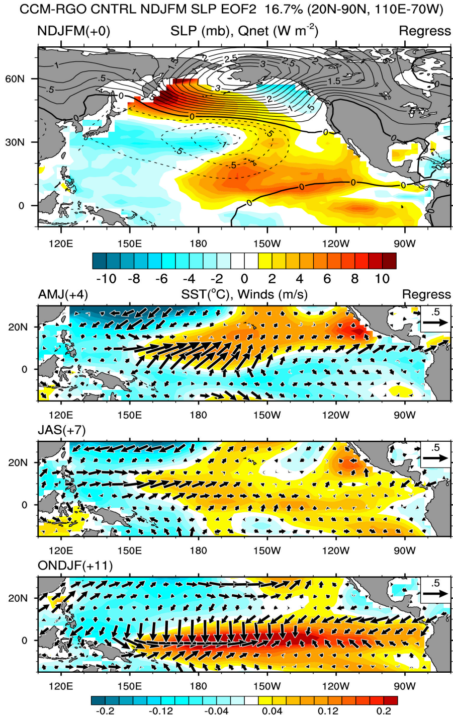
Fig. 1. The SFM simulated in a 100-year integration of the CCM3-RGO-ML model as indicated by: a) the concurrent regression of SLP [contour interval (CI) 0.25 mb per ] and Q_{net} [color shading interval (CSI) is 1 W m^{-2} per , positive into ocean) on the NPO time series - the second PC of SLP for EOFs computed over the North Pacific ( 20^{\circ}N-90^{\circ}N , 110^{\circ}E-70^{\circ}W ) during November-March; and lagged regressions of SST (shaded) and wind (vectors) in the tropical Pacific on the NPO time series for the following b) AMJ, c) JAS and d) ONDJF. The SST and wind scales are located at the bottom of the figure and the upper right corner of panels b)-d), respectively.
