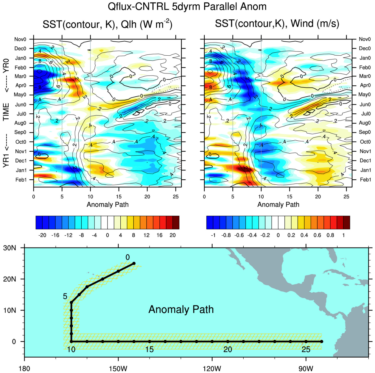
Fig. 6. Hövmoller diagrams of a) \Delta Q_{lh} (CSI is 2 \text{ Wm}^{-2} ) and b) \Delta U (CSI is 0.1 \text{ ms}^{-1} ); \Delta \text{SST} (CI is 0.1^\circ\text{C} ) is shown in both (a) and (b). (c) The Hövmoller path consists of three sections: i ) 25^\circ\text{N} , 155^\circ\text{W} extending southwest to 12^\circ\text{N} , 165^\circ\text{W} ; ii ) south along 165^\circ\text{W} to the equator and iii ) east along the equator to 85^\circ\text{W} ; corresponding to points i ) 0-5, ii ) 5-10 and iii ) 10-26, respectively along the entire transect. All values are derived from Exp-Cntrl 5-day running means averaged over three grid values including the points on and to either side of the transect line.
