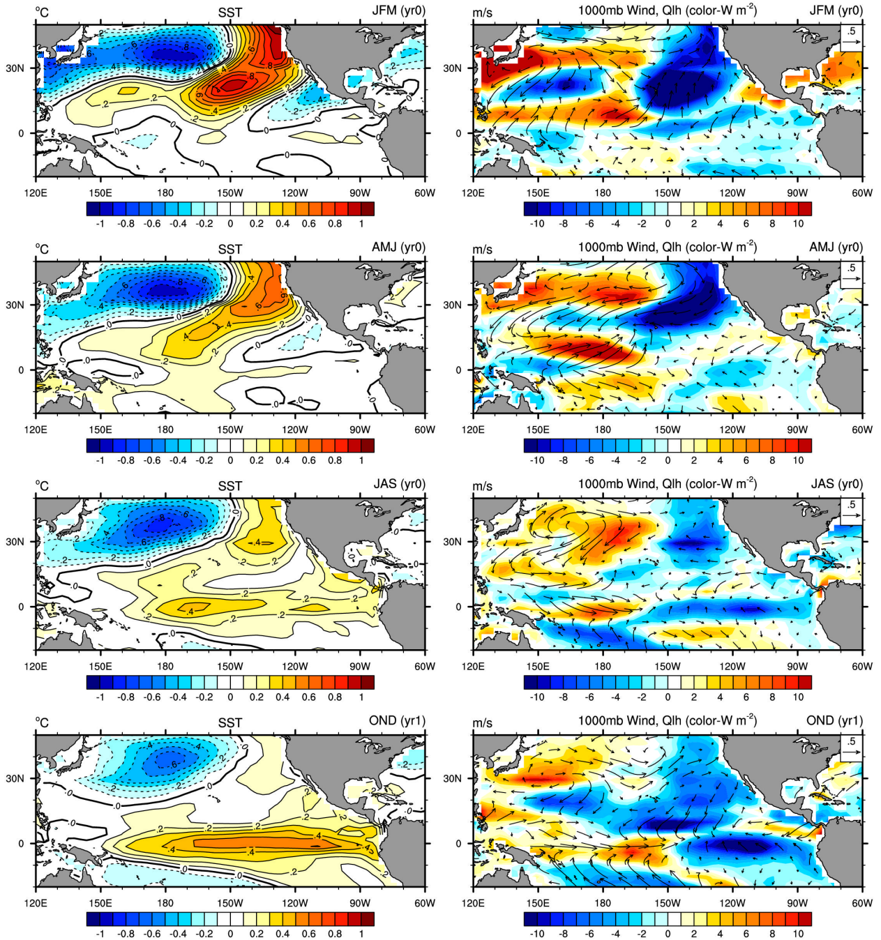
Fig. 3. The evolution of the response to the NPO-related forcing. The ensemble mean difference ( \Delta ) between the “Qflux” experiment (Exp) and control (Cntrl) simulations for (left) SST (CI is 0.1^\circ\text{C} ) and (right) 1000 mb wind (vectors, \text{m s}^{-1} ) and latent heat flux ( Q_{lh} \text{Wm}^{-2} ). The response is shown, from top to bottom, for JFM(0), AMJ(0), JAS(0) and OND(1), where 0 denotes the initial year of the integration and 1 the following year.
