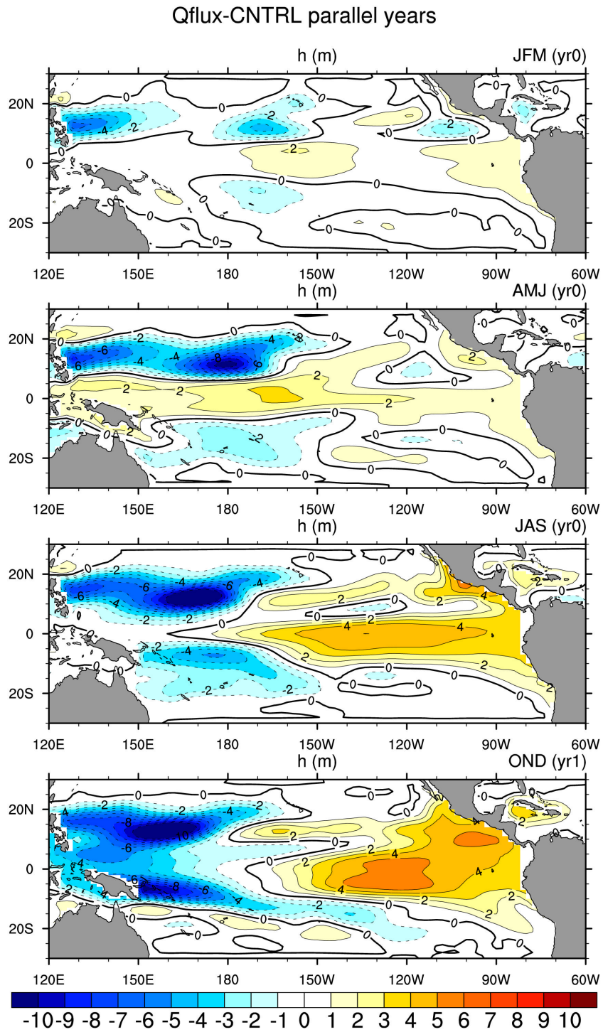
Fig. 4. As in Fig. 3, but for the thermocline depth ( \Delta h , CI & CSI are 1m) response.
