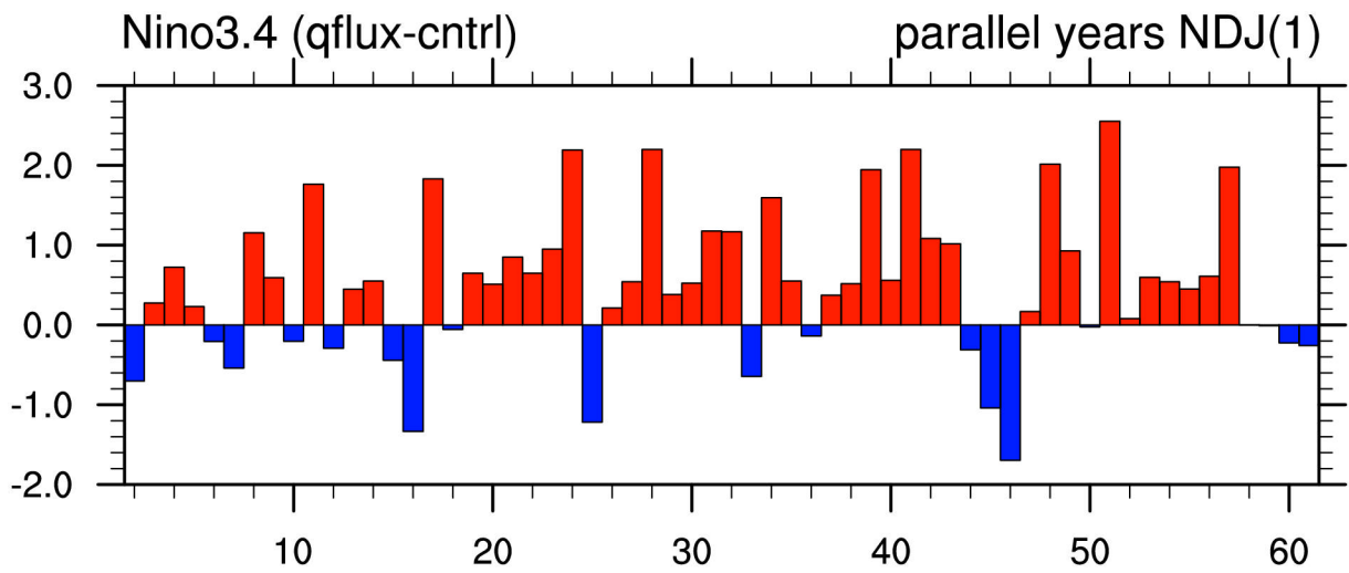
Fig. 8. Bar chart of the Exp – Cntrl ( \Delta ) SST ( ^{\circ} C) during NDJ(1) in the Nino 3.4 region for each of the 60 branch simulations numbered by the order the year they occur in the control run.
