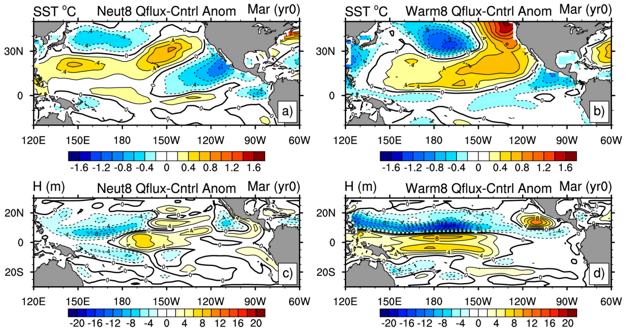
Fig. 11. The \Delta SST (CI &CSI are 0.2^{\circ}\text{C} ) for the a) neutral and b) warm composite, and the \Delta h (CI &CSI are 2 m) for the c) neutral and warm composite d) in Mar(0).
