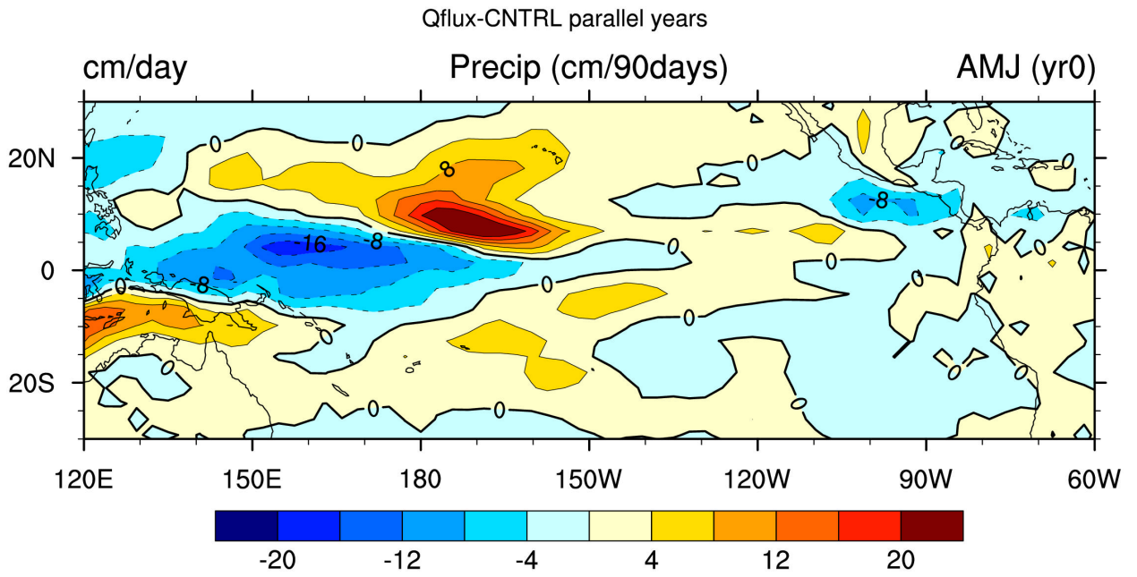
Fig. 5 The response in precipitation ( \Delta P , CI&CSI are 4 cm per 90 days) during AMJ(0).
