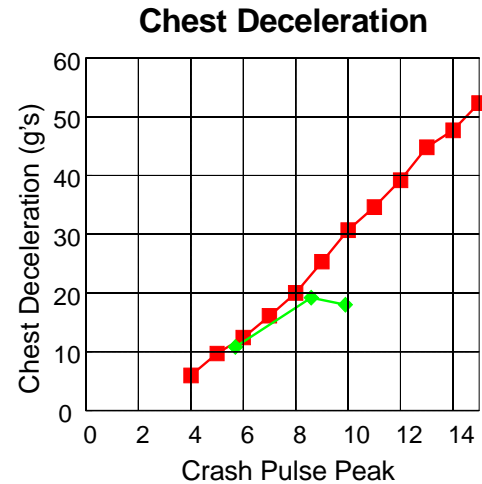
Figure 6-2. Chest Deceleration
