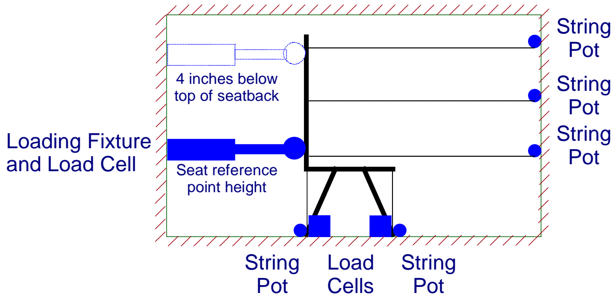
Figure A-3. Static Test Arrangement.
