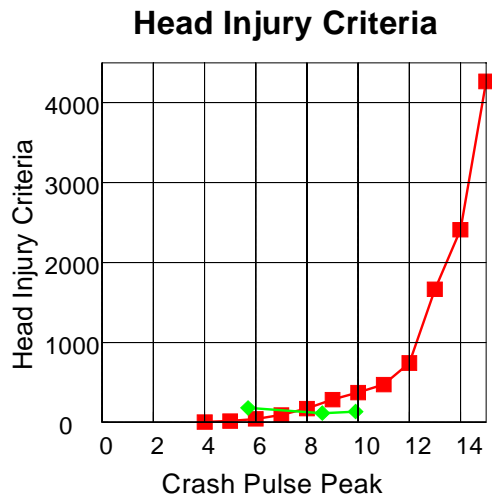
Figure 6-1. Head Injury Criteria
