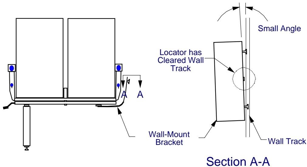
Figure 5-7. Schematic of Wall Bracket Attachment
