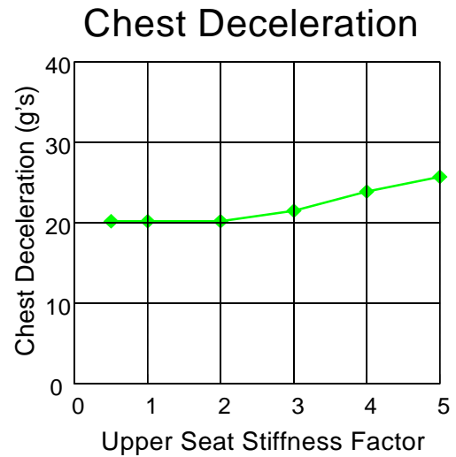
Figure 6-8. Chest Deceleration
