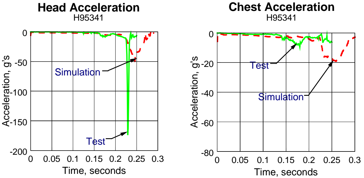
Figure D-7. Acceleration Time Histories for Test 7 Conditions
