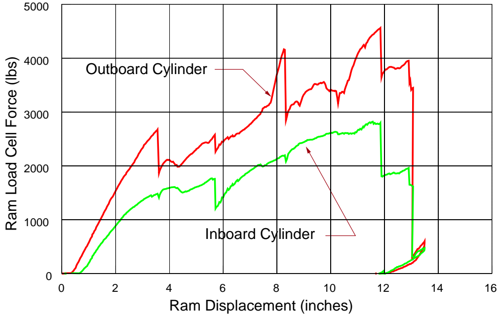
Figure 5-3. Knee-Load Test, Measured Force vs. Displacement
