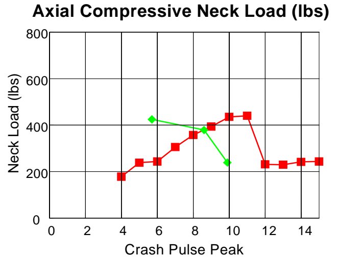
Figure 6-4. Axial Compressive Neck Load
