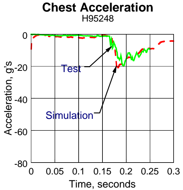
Figure D-3. Acceleration Time Histories for Test 3 Conditions
