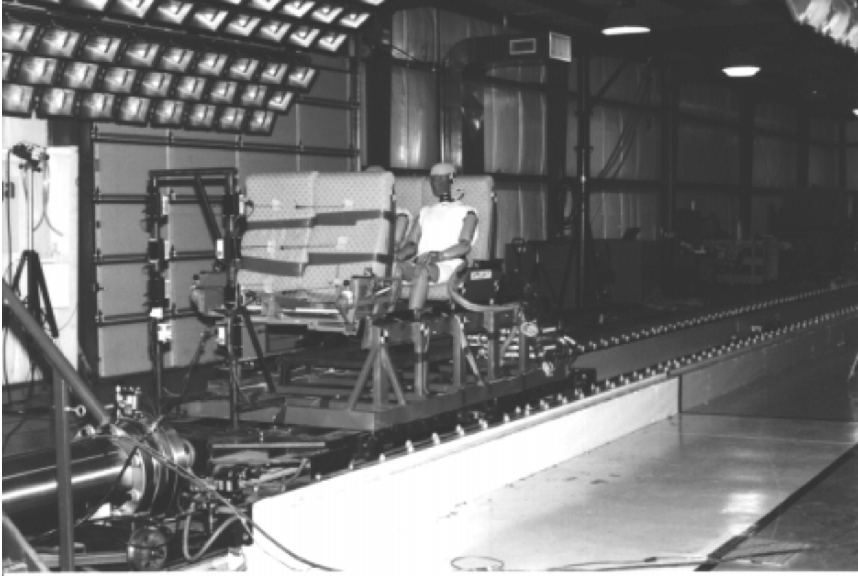
Figure 4-3. Dynamic Test Sled
