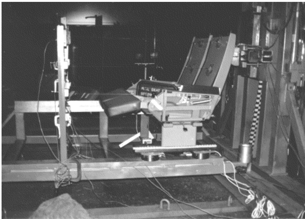
Figure 4-1. Quasi-Static Test Fixture
