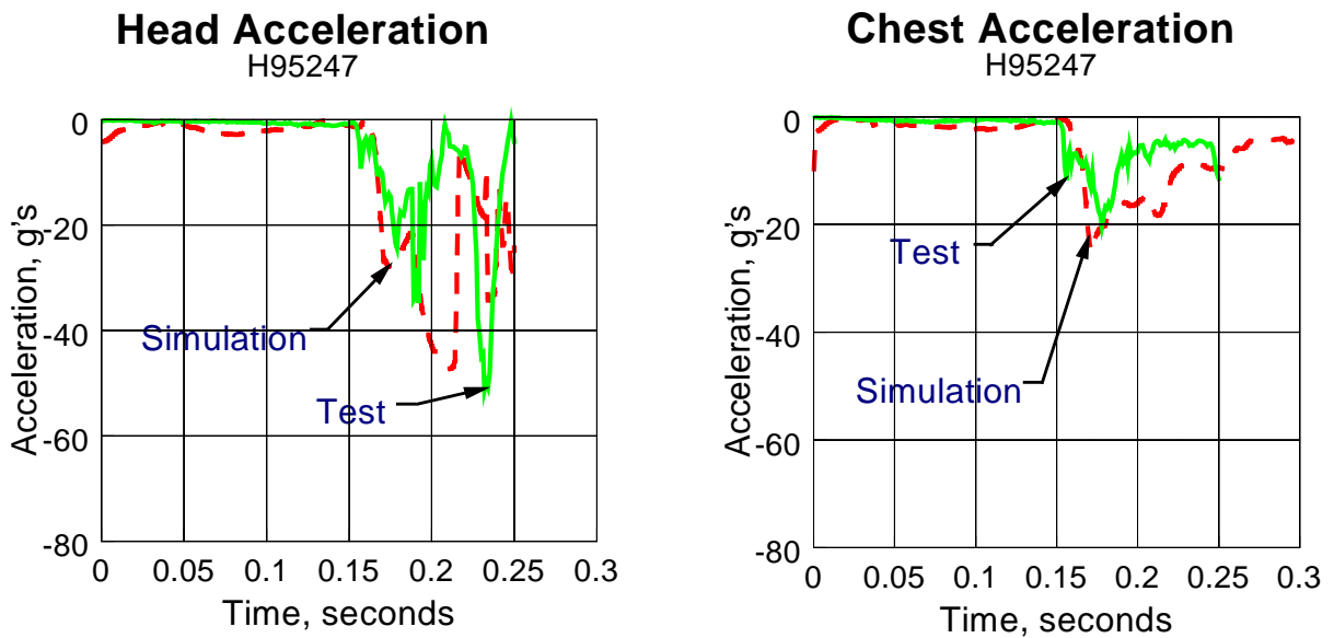
Figure D-2. Acceleration Time Histories for Test 2 Conditions
