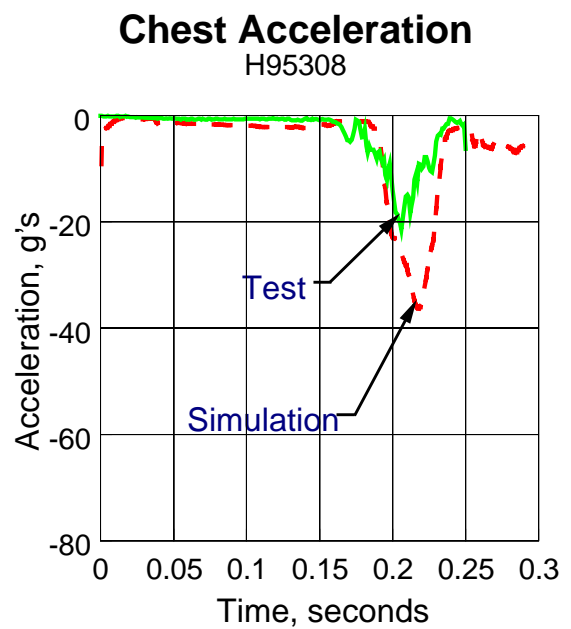
Figure D-4. Acceleration Time Histories for Test 4 Conditions
