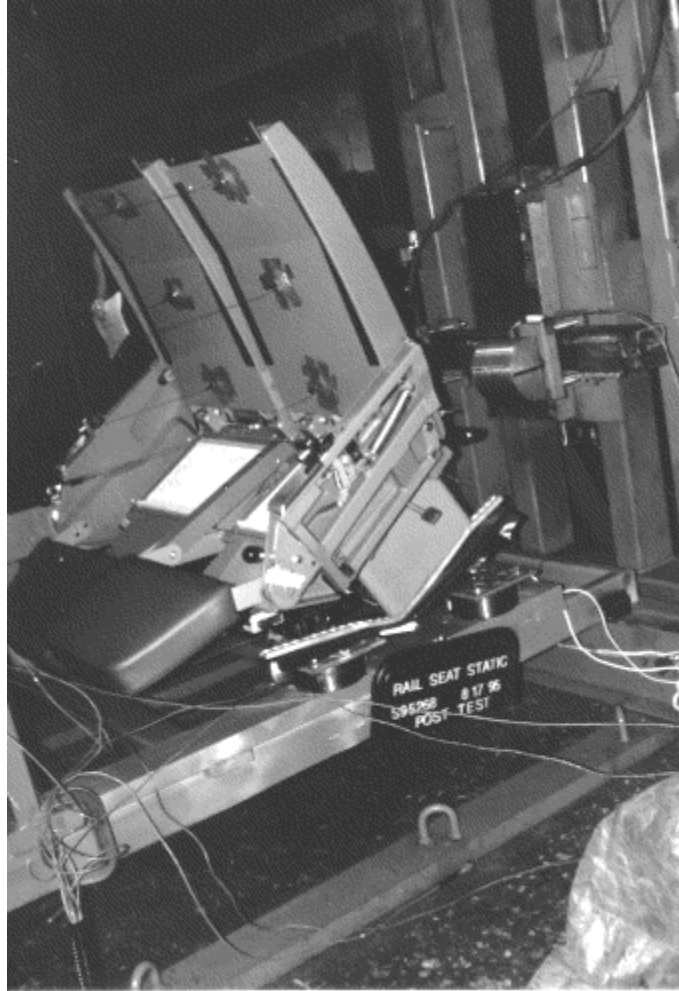
Figure 5-4. Knee-Load Quasi-Static Test, Seat Pair Post-test Condition
