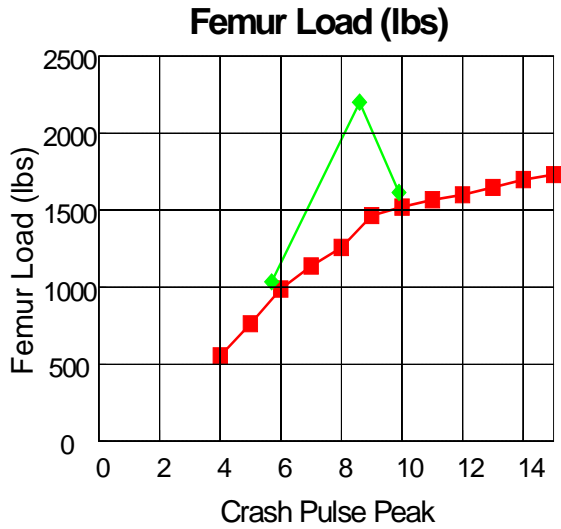
Figure 6-3. Femur Load
