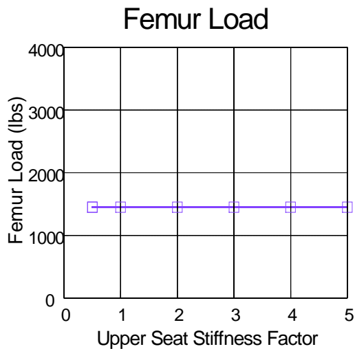
Figure 6-9. Femur Load
