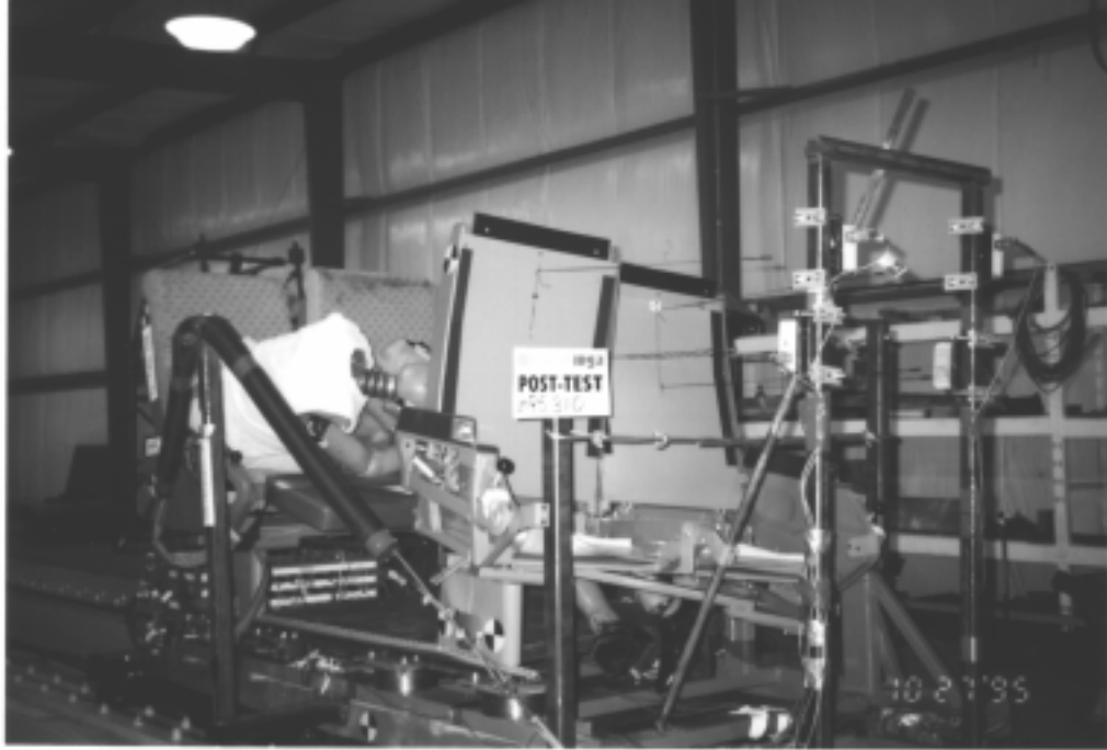
Figure 5-13. Dynamic Test 5, Post-test Condition
