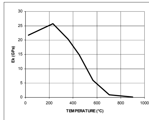
Figure A7. Hardening modulus versus temperature (°C).
