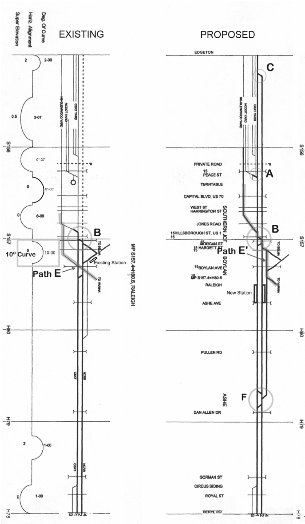
Figure 6-7: Schematic of Raleigh
