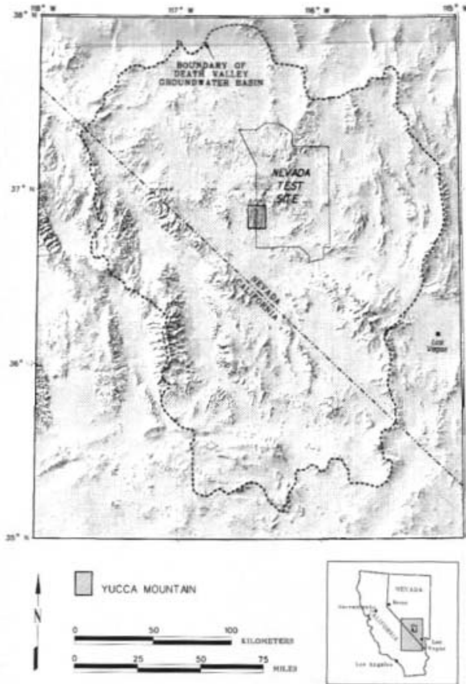
Figure 7-24. Death Valley Ground Water Flow System (USG96a)
