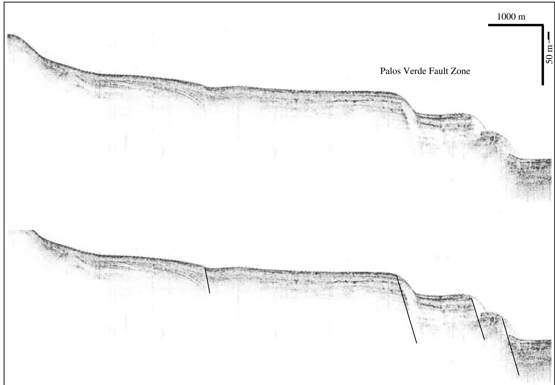
Figure 6. Example of 3.5 kHz bathymetry profiler record from Line LARSE04 across Palos Verde fault zone.
