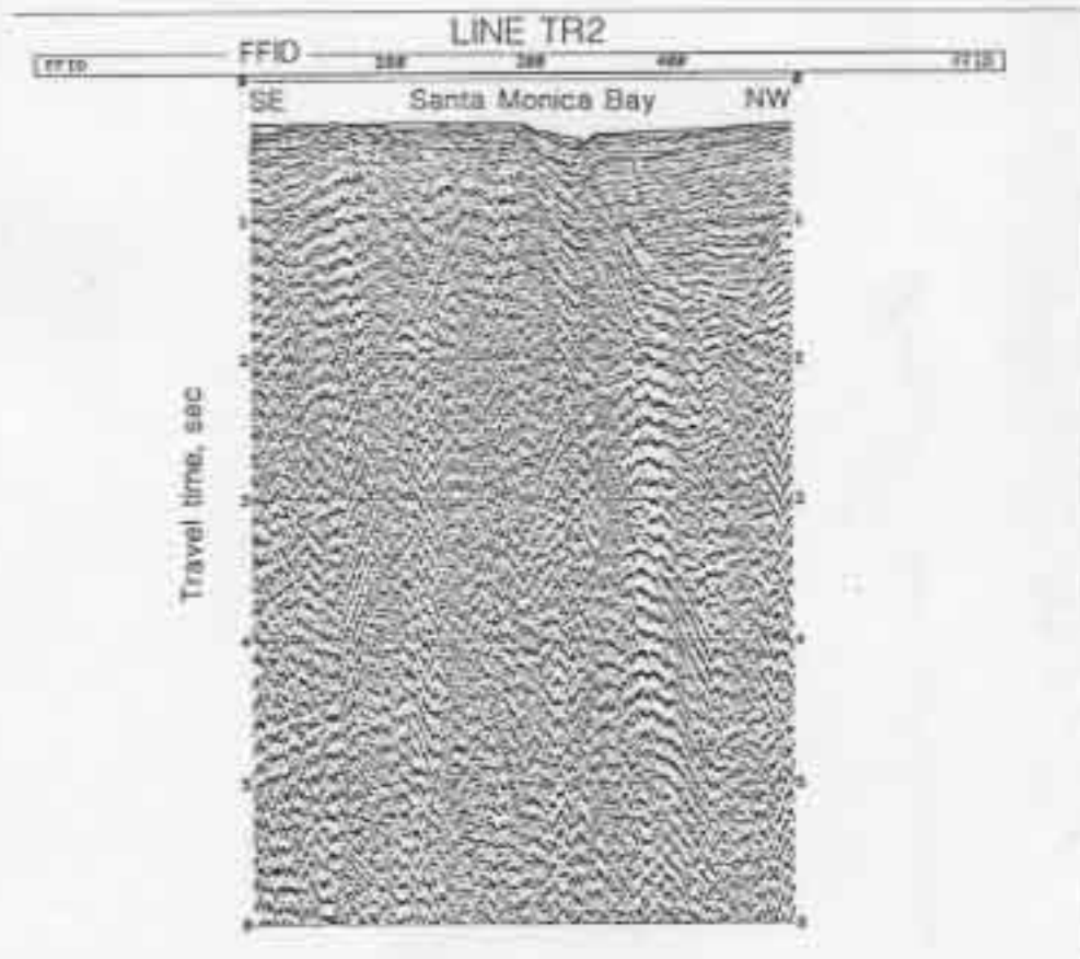
Fig. 9. Near-trace (ch. 150) constant offset section for Lines TR1a and b, TR2, and TR3. As described in text processing included hand pass filtering, automatic gain control (AGC), and water column mute.
