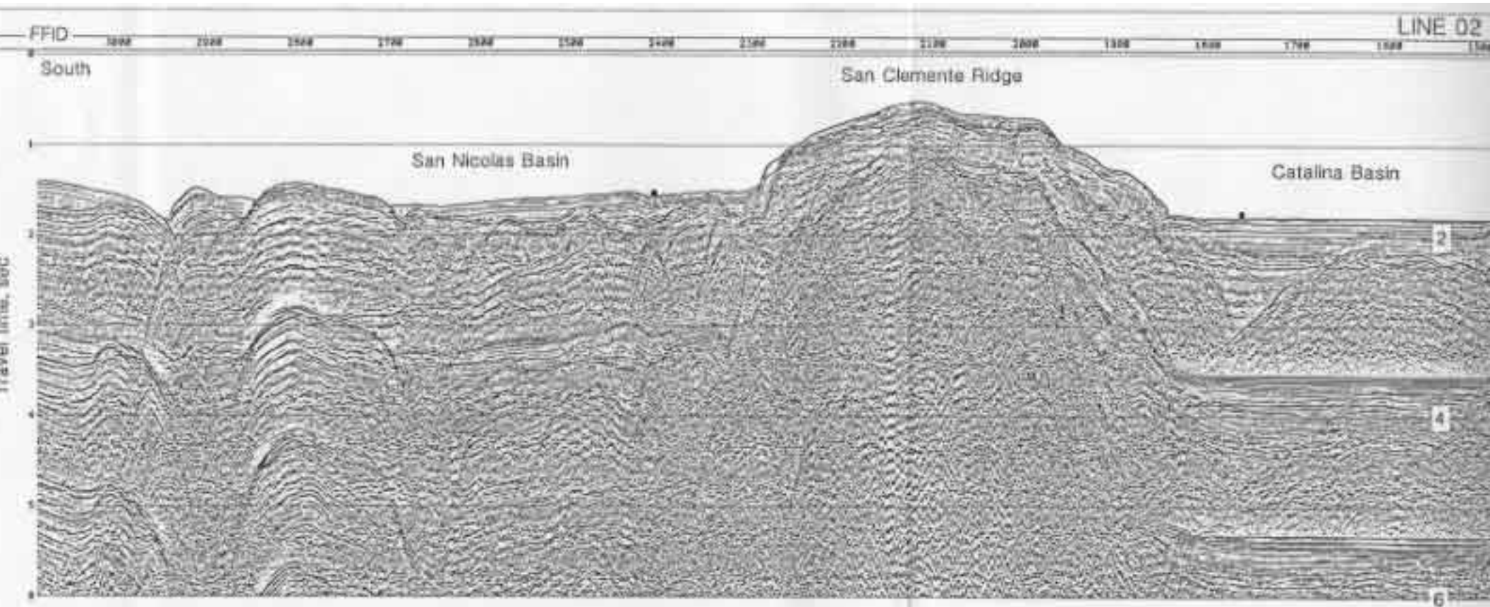
Fig. 7. Near-trace (ch. 150) constant offset section for Lines LAR5E01R and LAR5E02. As described in text processing included band pass filtering, automatic gain control (AGC), and water column mute.
