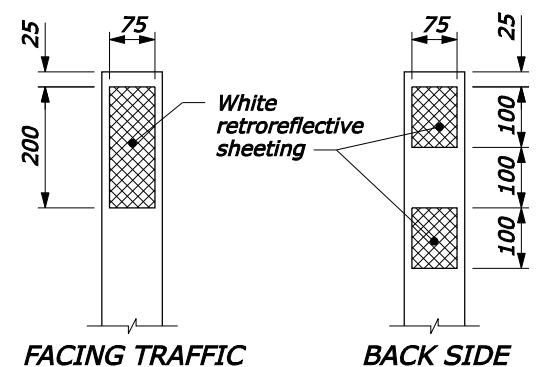
FLEXIBLE DELINEATOR GUARDRAIL MOUNTED OPTION (Use only with wood guardrail posts)
