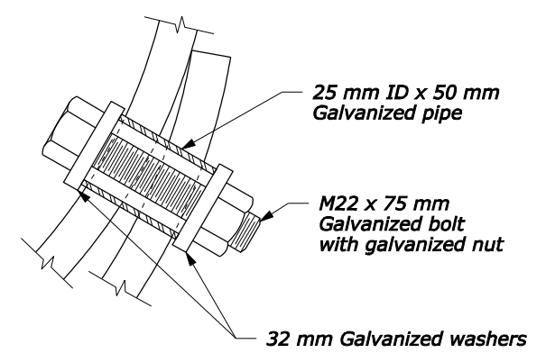
BOLT DETAIL
