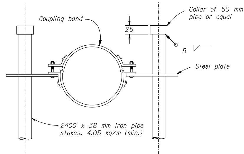
ANCHOR ASSEMBLY
