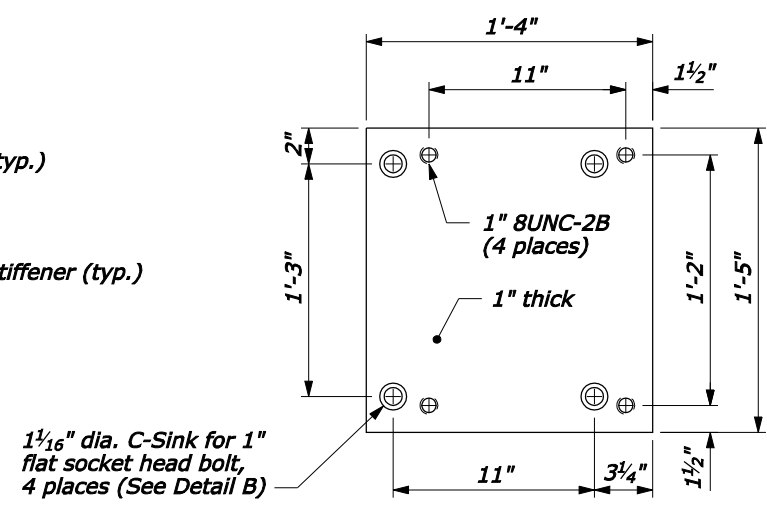
TOP CLAMP PLATE
