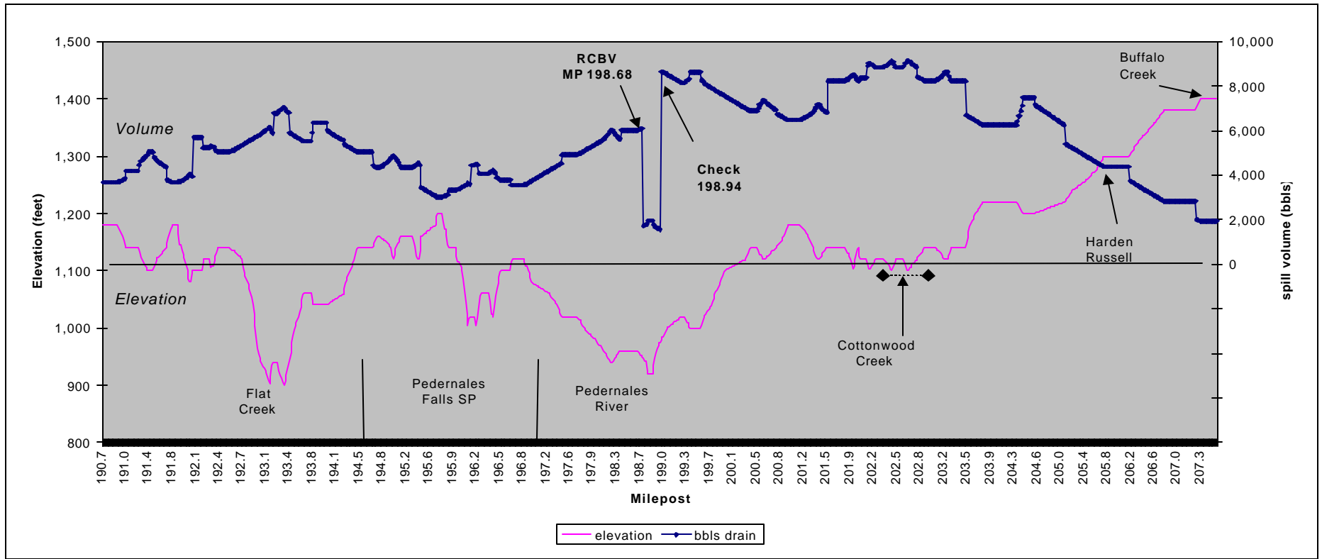
Figure 7-2. Spill Volumes and Elevations in Pedernales Watershed Along Longhorn Pipeline
