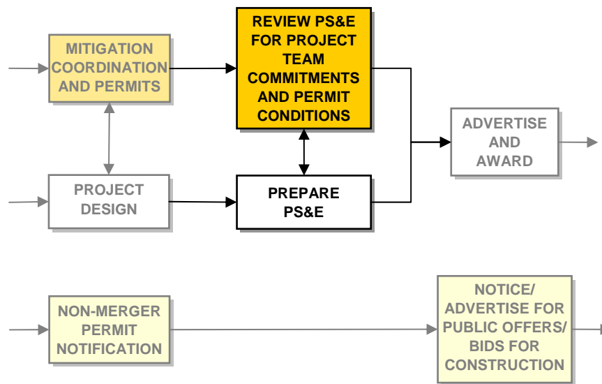
Exhibit 3.4–K REVIEW PS&E
