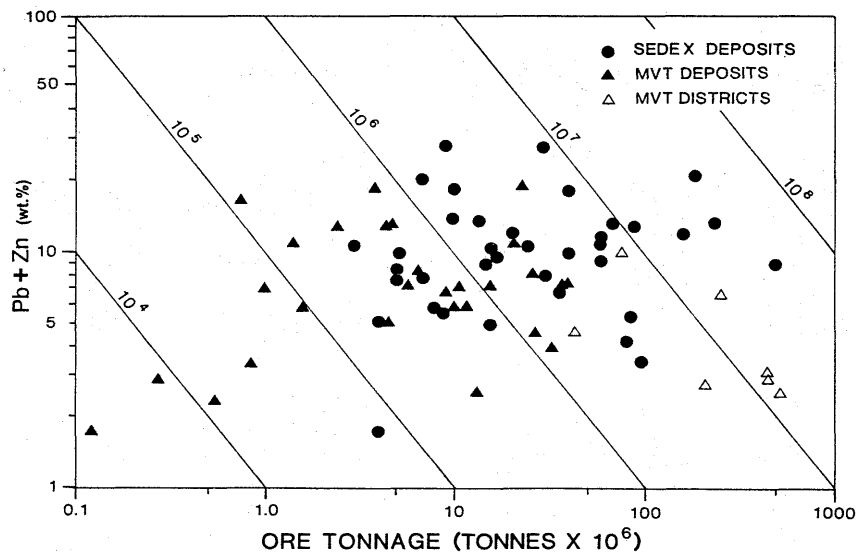
Figure 2. Grade-tonnage for MVT deposits and districts and for sedimentary exhalative deposits. Diagonal lines represent total tonnage of contained lead and zinc (adapted from Sangster, 1990).
