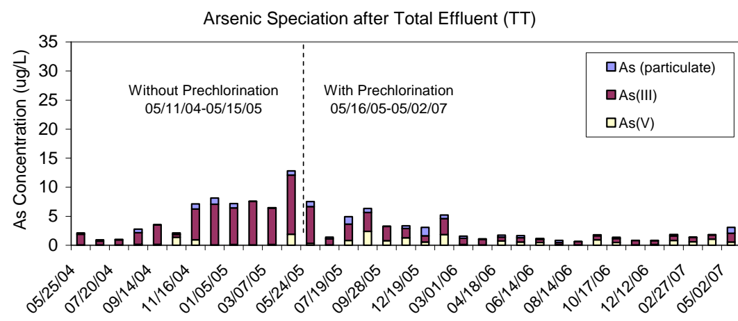
Figure 4-12. Concentrations of Arsenic Species at Wellhead, After Chlorination, and After Combined Effluent
