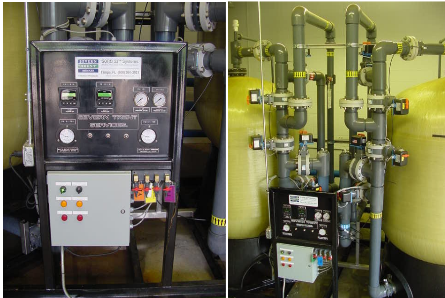
Figure 4-6. System Components (Control Panel & Color Coded Sample Taps [left]; and APU-300 System Valve Tree [right])
