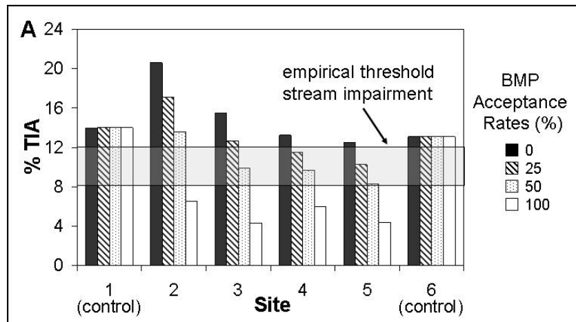
Figure 2.2.2 Percent TIA given 0, 25, 50, and 100% landowner acceptance rates of rain gardens and rain barrels.
