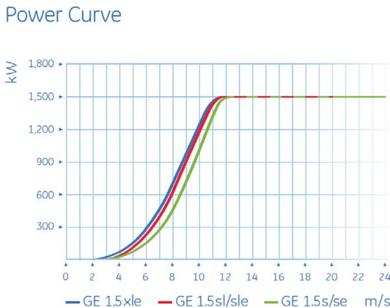
Figure 2. Wind power curve for a GE 1.5se (1.5 MW) wind turbine. Source: http://www.gepower.com/prod_serv/products/wind_turbines/en/downloads/ge_15_brochure.pdf
