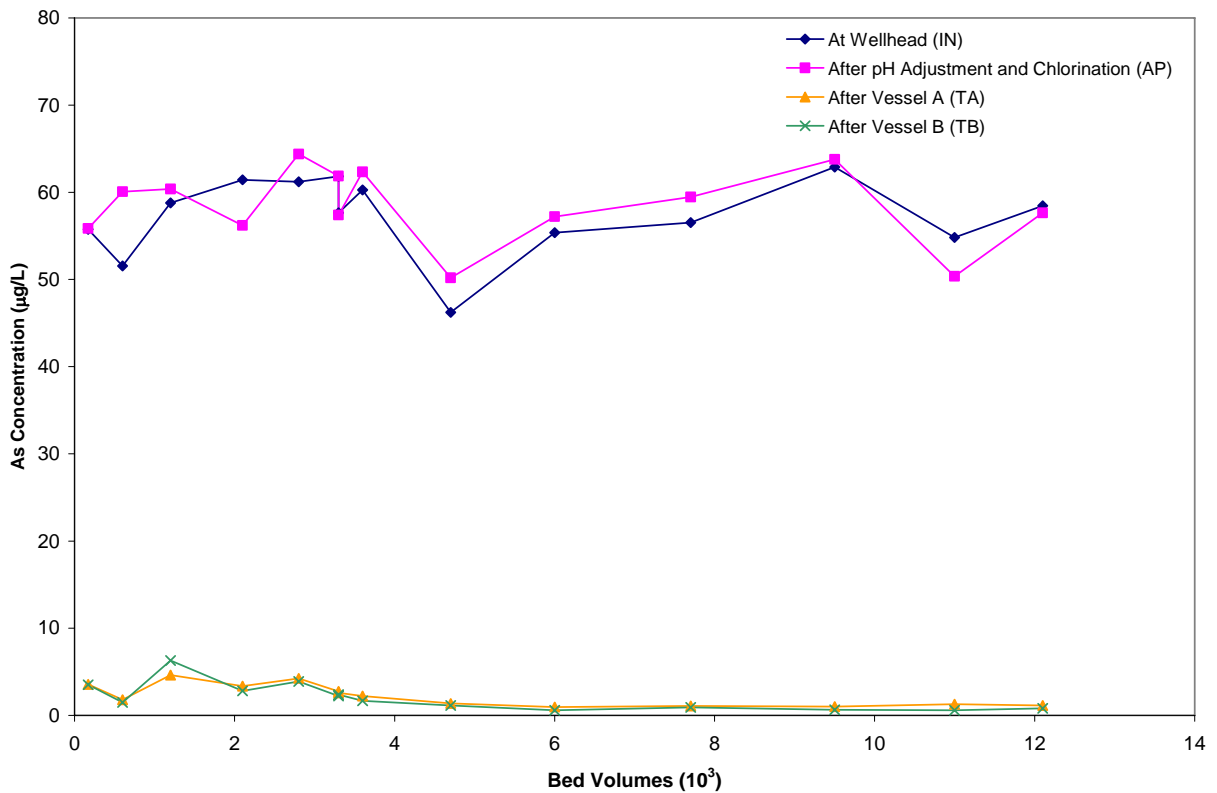
Figure 4-15. Total Arsenic Breakthrough Curves (Based on 22 ft 3 of Media in Each Vessel)
