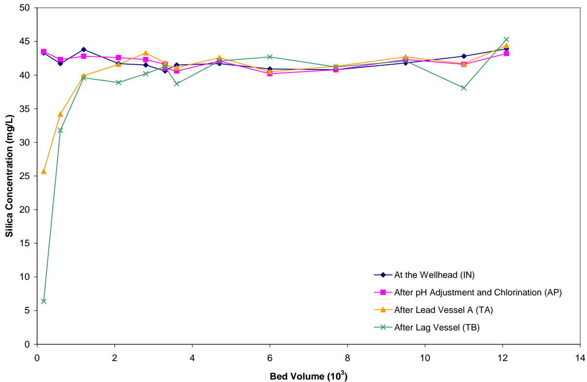
Figure 4-16. Silica (as SiO 2 ) Breakthrough Curves (Based on 22 ft 3 of Media in Each Vessel)
