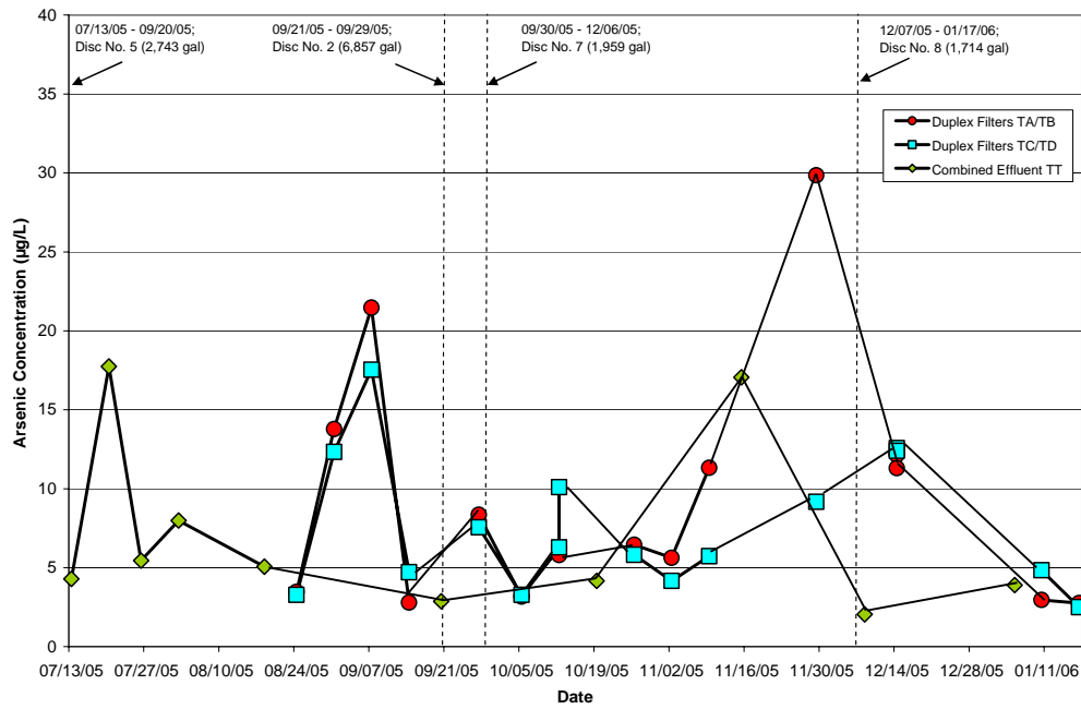
Figure 4-9. Total Arsenic Concentrations at TA/TB, TC/TD, and TT Sampling Locations
