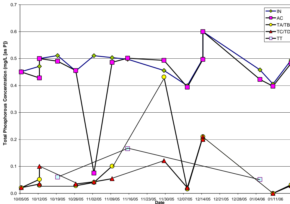
Figure 4-14. Total Phosphorous Concentrations at IN, AC, TA/TB, TC/TD and TT Sampling Locations
