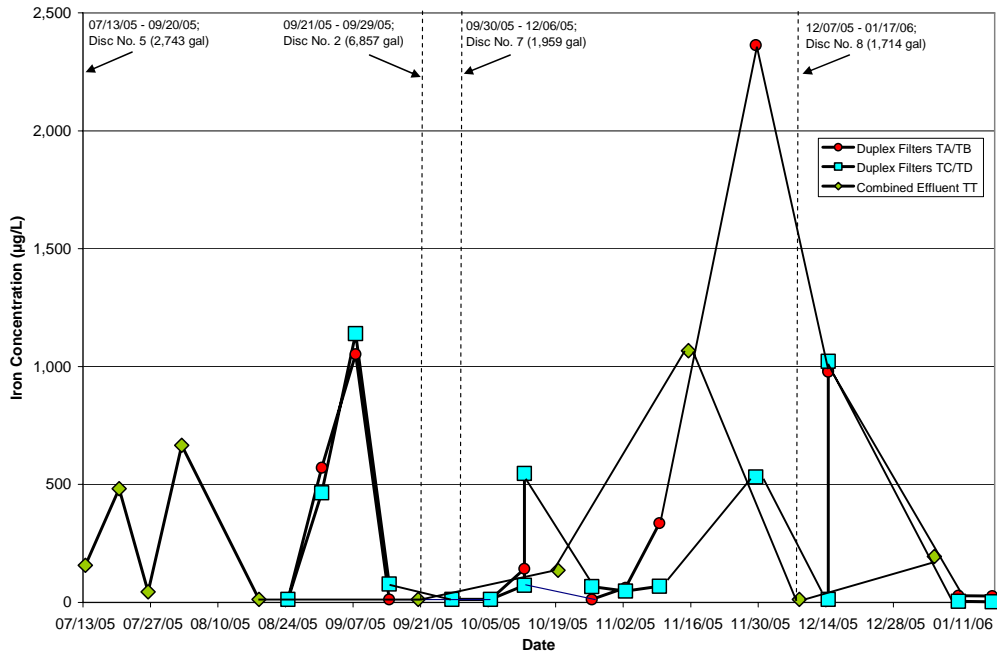
Figure 4-10. Total Iron Concentrations at TA/TB, TC/TD, and TT Sampling Locations
