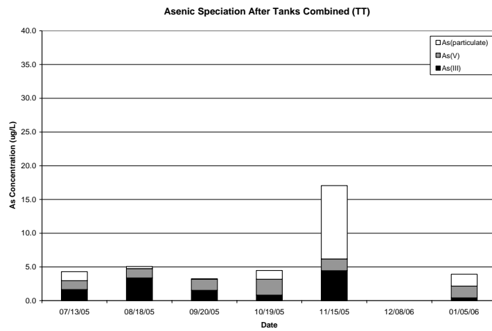
Figure 4-8. Concentrations of Arsenic Species at IN, AC, and TT Sampling Locations
