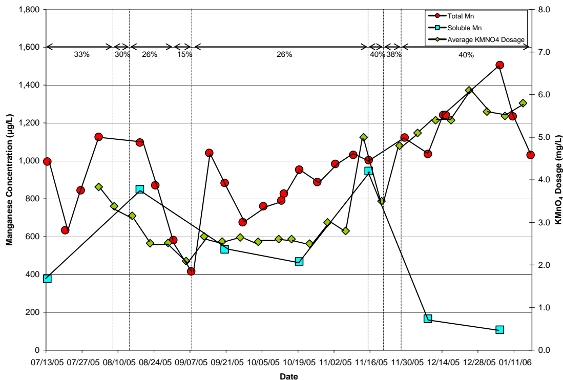
Figure 4-11. Total and Soluble Manganese Concentrations at AC Sampling Location
