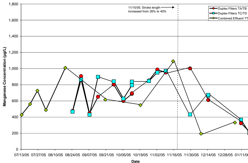
Figure 4-12. Total Manganese Concentrations at TA/TB, TC/TD, and TT Sampling Locations
