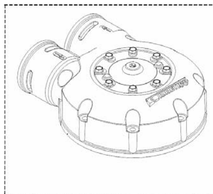
Figure 4-6. Kinetico's Mach 1250 Control Valve
