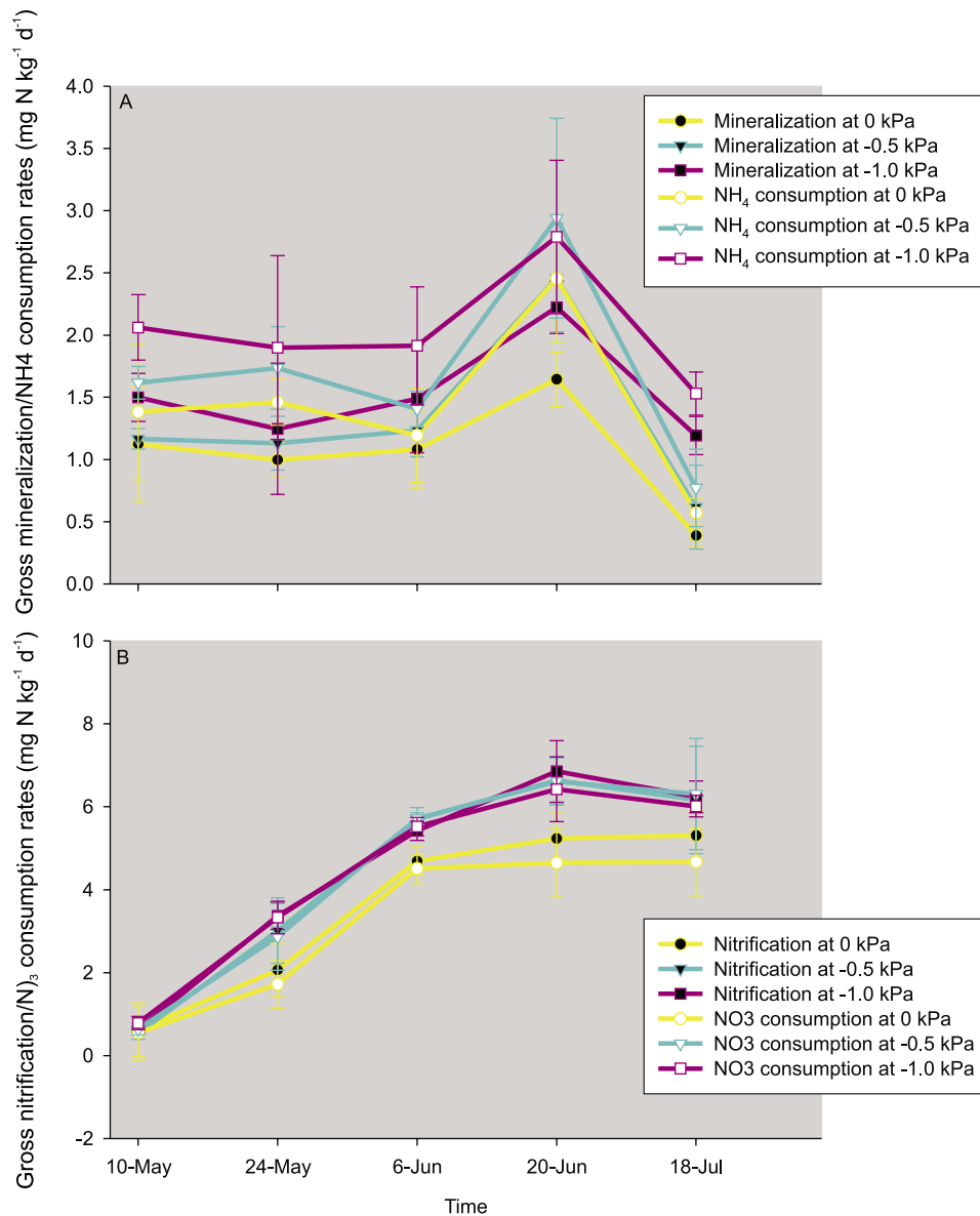
Figure 8. Gross mineralization and NH 4 + consumption rates (A) and gross nitrification and NO 3 - consumption rates (B) from old-field soils under three different water potentials measured under laboratory conditions. Vertical bars indicate \pm standard error of mean.
