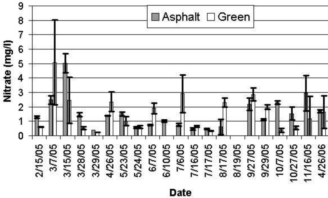
Figure 4-11 Nitrate concentration in runoff from green and flat asphalt roofs
