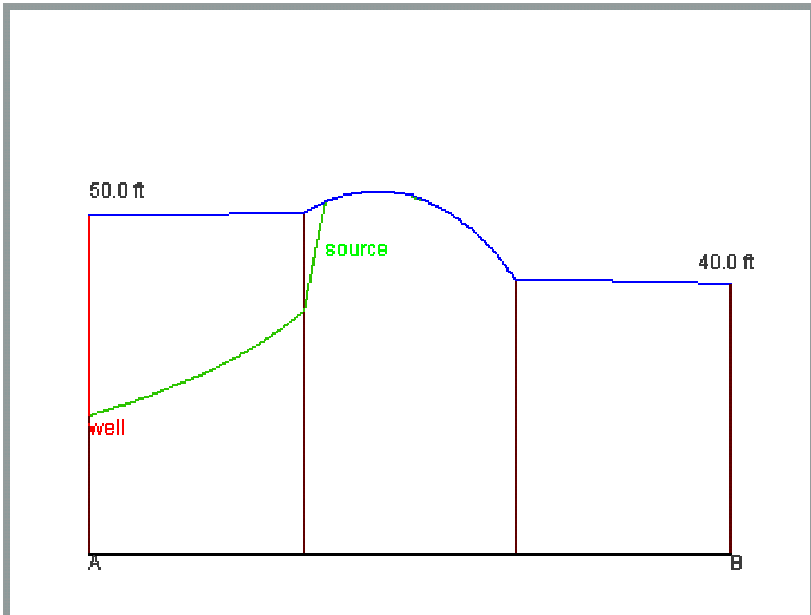
Figure 36 Water table mounding due to unequal recharge and hydraulic conductivity.
