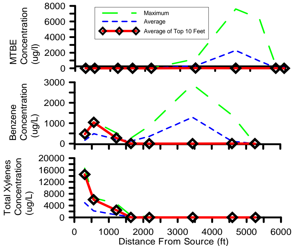
Figure 2 Consequences of sampling only the top ten feet of the aquifer at East Patchogue, New York. The MTBE plume would disappear (top); the benzene plume would be shortened by two thirds; and the total xylenes plume appears at the same length because its extent did not reach the gravel pit where diving dominates the contaminant distribution.
