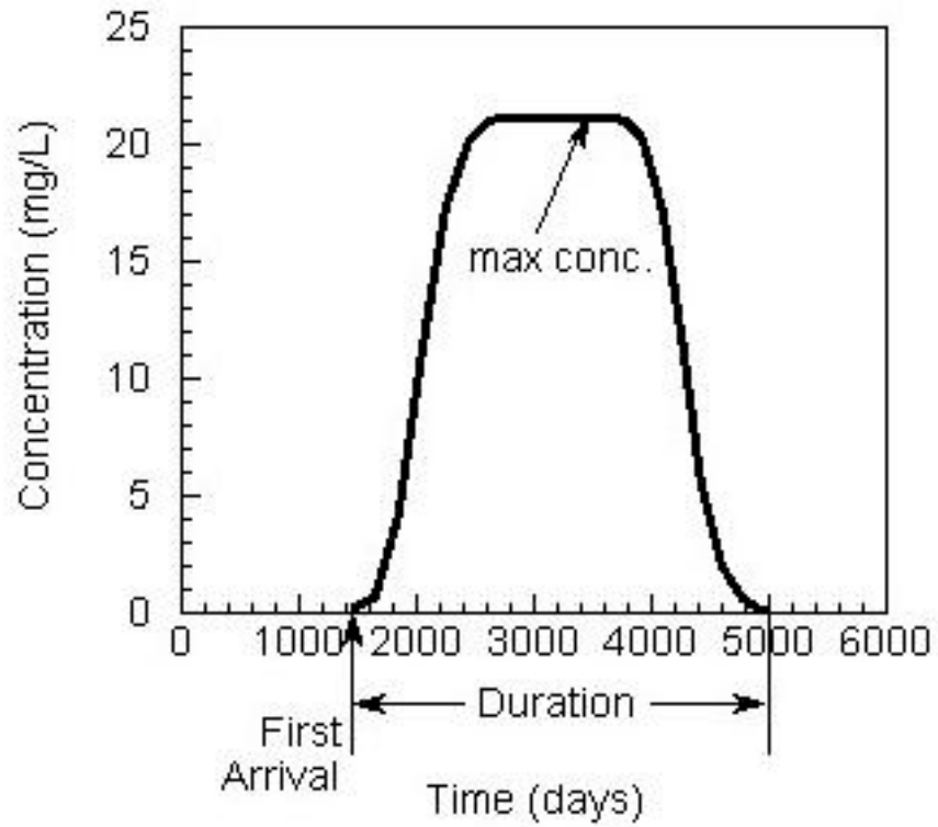
Figure 20 Illustration showing the relationship between the first arrival time, maximum concentration and duration of contamination. The first arrival time and duration are determined relative to a given threshold concentration, that is usually a maximum contaminant level or other concentration of concern.
