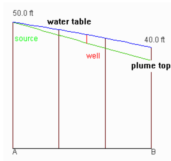
Figure 16 Plume Diving calculator graphical output.
