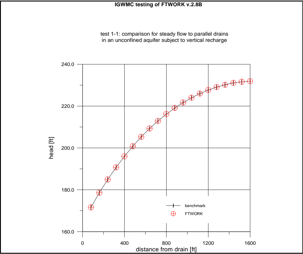
Figure 1.1.1. Comparison of heads with distance from a fixed head boundary for steady flow to parallel drains in an unconfined aquifer subject to vertical recharge.
