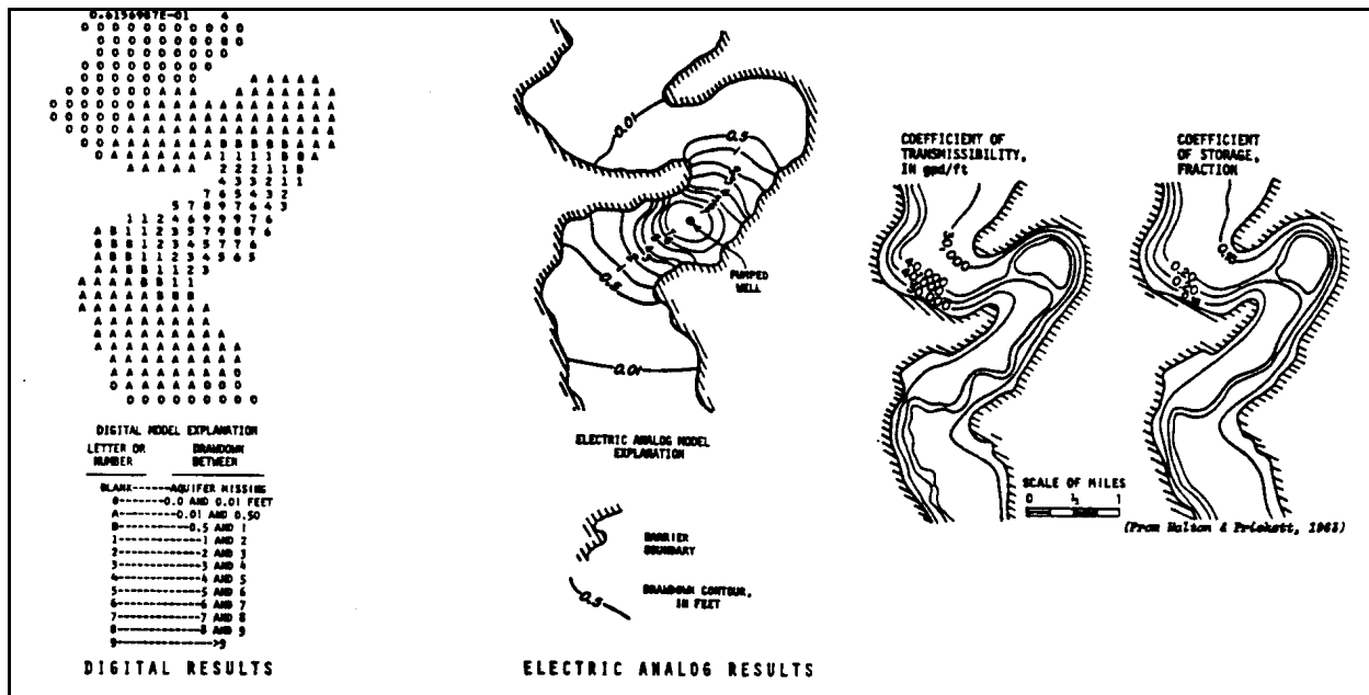
Figure 2-2. Example of comparison of numerical and laboratory analog solutions (from Prickett and Lonquist, 1971)
