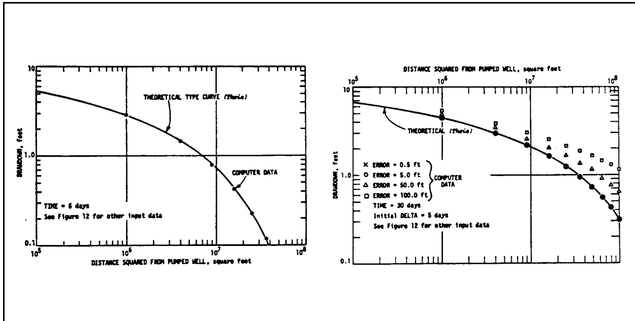
Figure 2-1. Examples of comparison of numerical and analytical solutions (from Prickett and Lonquist, 1971)
