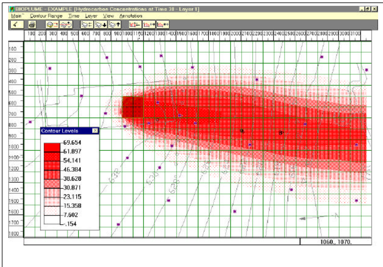
Figure 1. Example of 2D graphical output from Bioplume III showing a modeled hydrocarbon plume.
