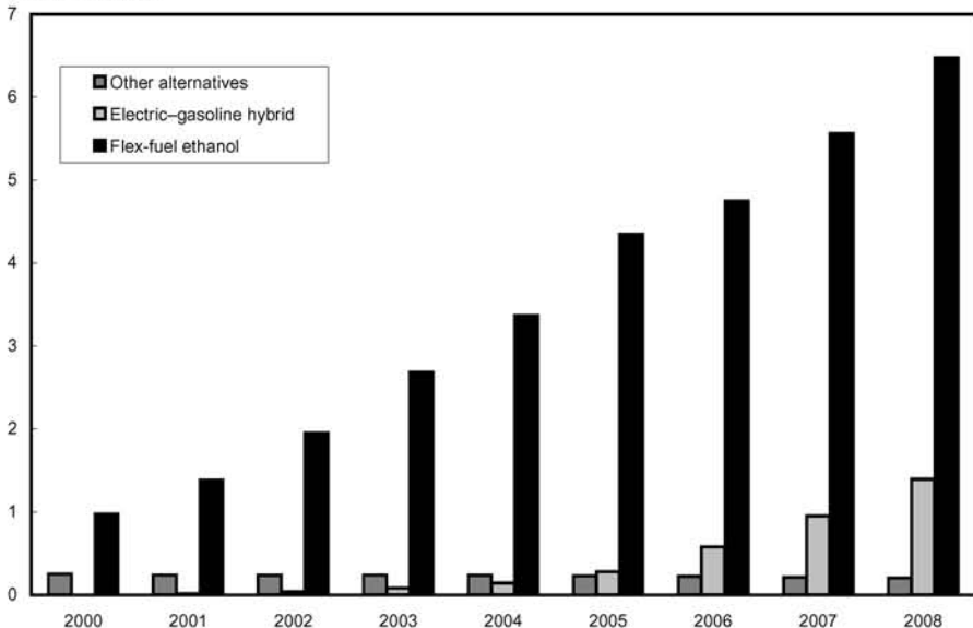
Chart 3-2 Alternative Fuel Light-Duty Vehicles in the U.S. Fleet
