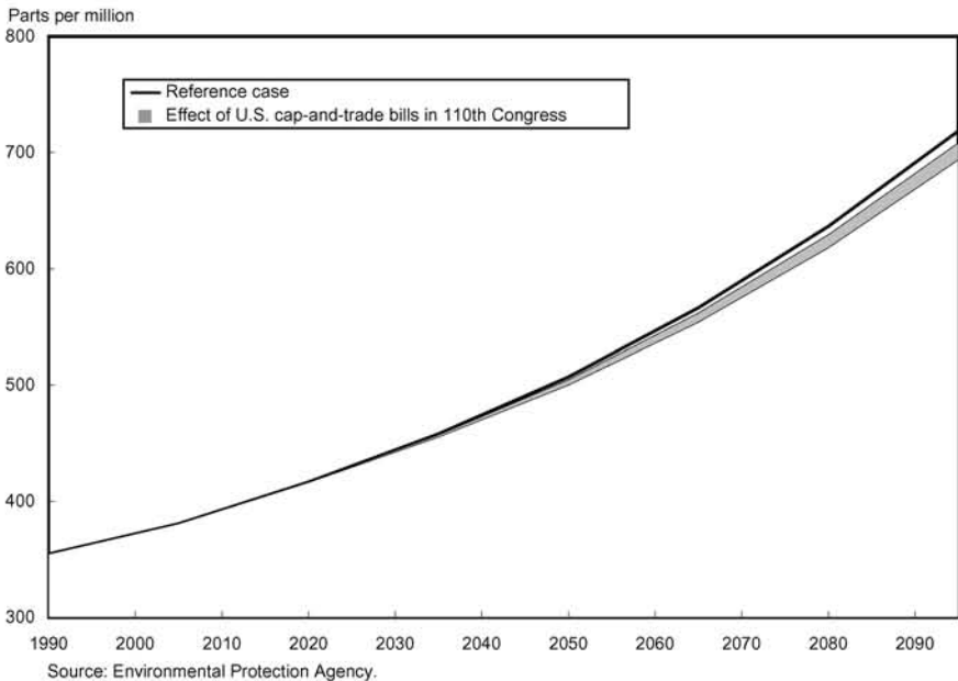
Chart 3-6 Global CO 2 Concentrations
