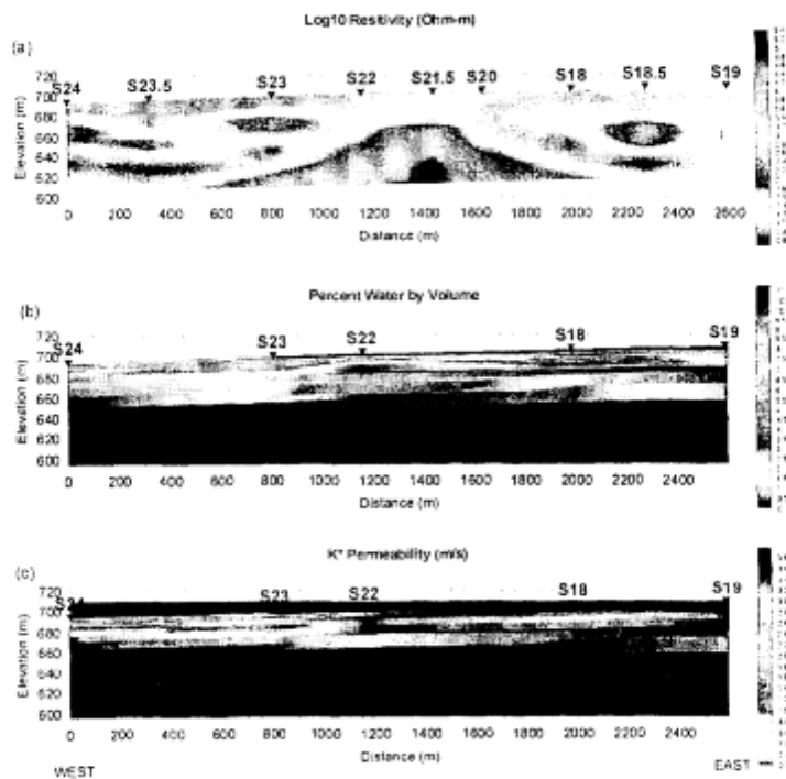
Figure 1. Results of TDEM and NUMIS soundings along the E-W profile at Ash Meadows, Nevada (a) Inverted TDEM data in \log_{10} (resistivity) (b) NUMIS percent Water content, and (c) NUMIS permeability (m/s).
