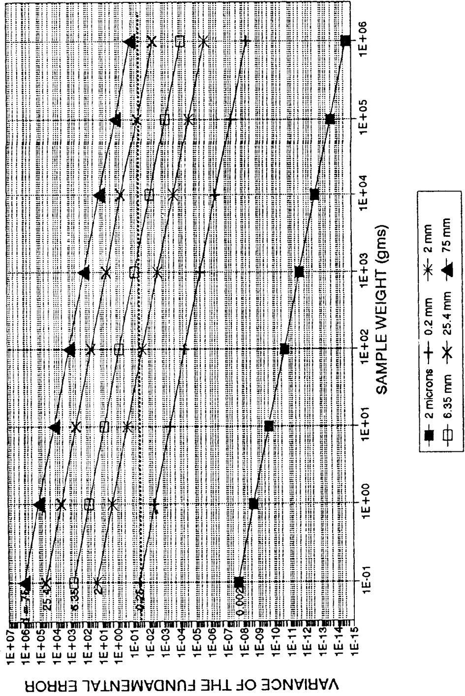
FIGURE A7: SAMPLING NOMOGRAPH FOR SOILS C = 250
