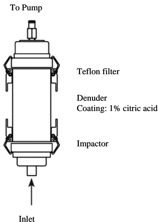
Figure 3-2. Reference Method Sampling Cartridge
