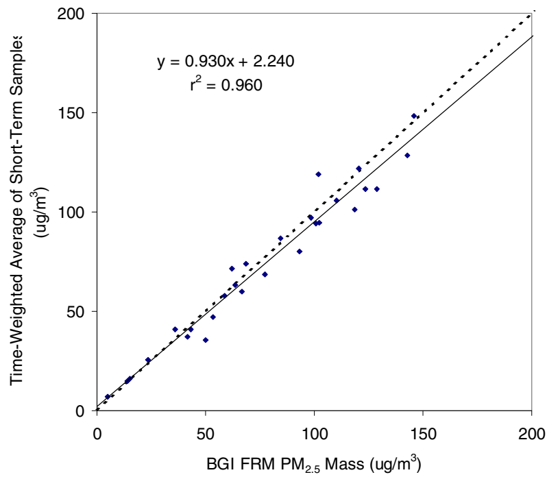
Figure 6-7. Correlation Plot for the Time-Weighted Average of the Short-Term Samples and the PM 2.5 FRM for Phase II
