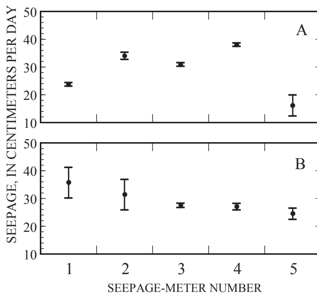
Figure 16. Seepage heterogeneity as indicated by five 20.25-cm-diameter seepage meters installed in tank 2 before (A) and after (B) draining, stirring, and refilling water in the tank, and restirring the sand bed in an attempt to reduce heterogeneity.
