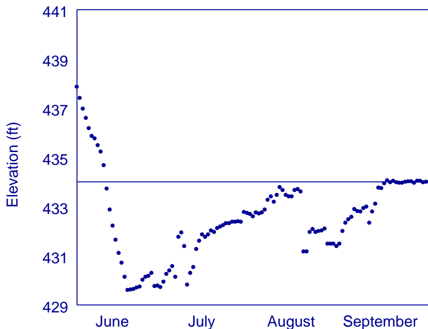
Figure 1. Water levels just upriver of Dam 25 during the summer of 1995.
