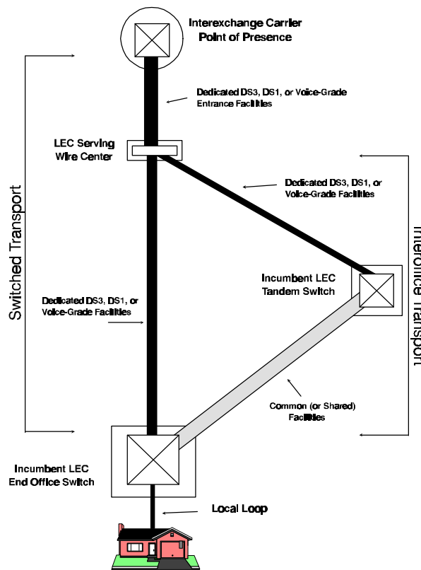
FIGURE 1: INCUMBENT LEC SWITCHED TRANSPORT NETWORK
