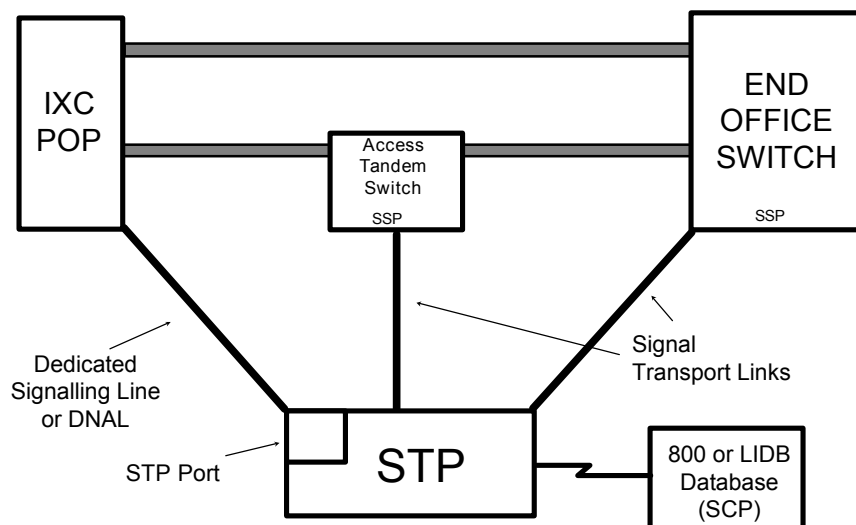
FIGURE 2: SS7 NETWORK
