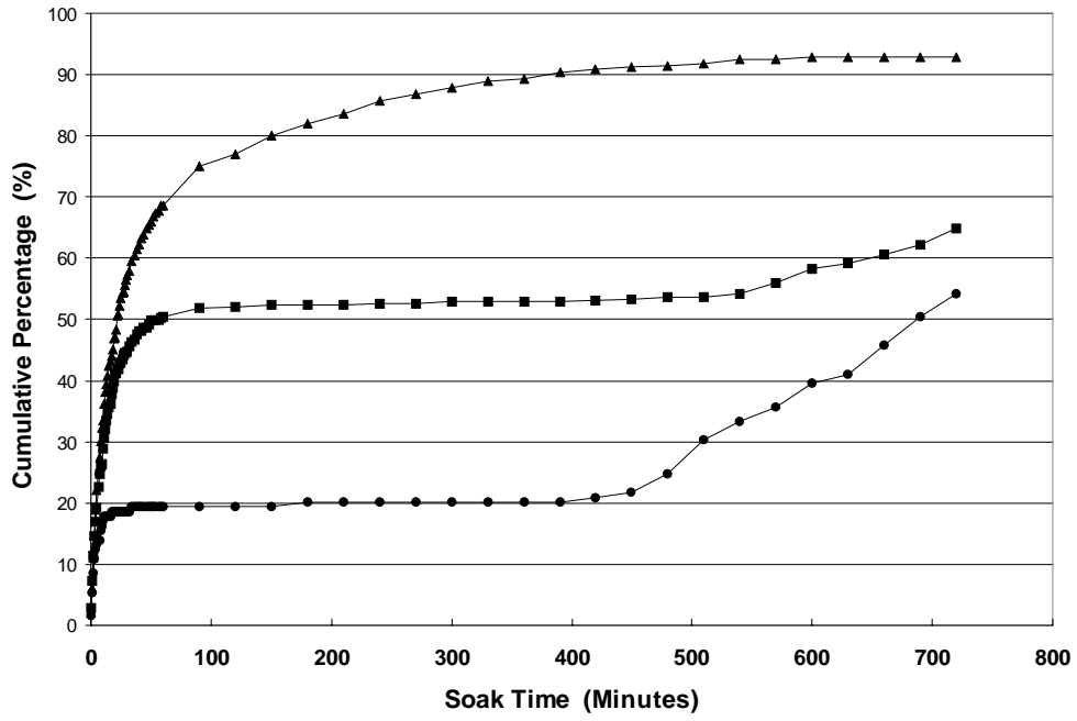
Figure 1 Cumulative Soak Length Distribution for Selected Hourly Groups (Soaks are Prior to Vehicle Start)
