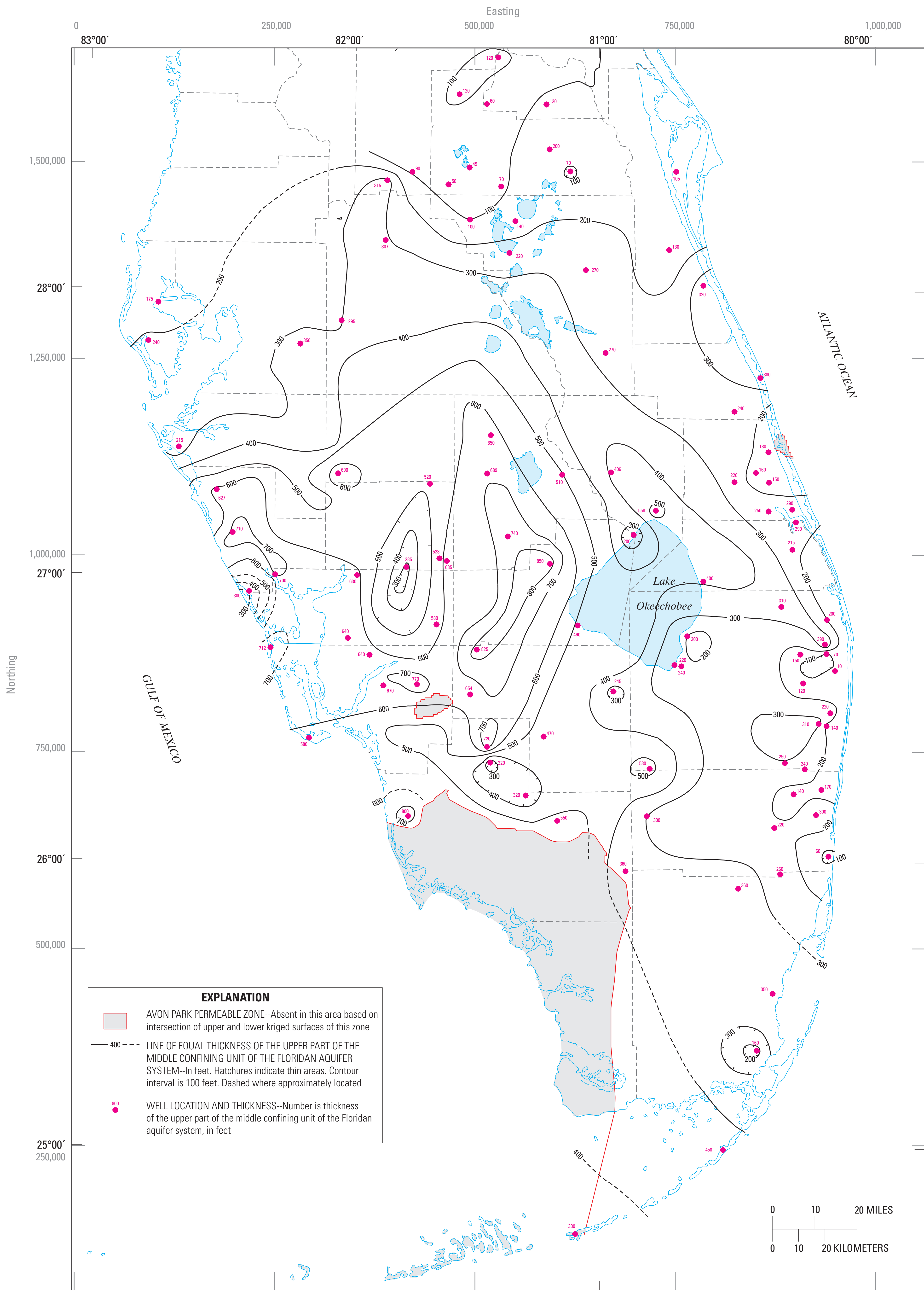
Figure A7. Thickness of the upper part of the middle confining unit (MCI) of the Floridan aquifer system.
