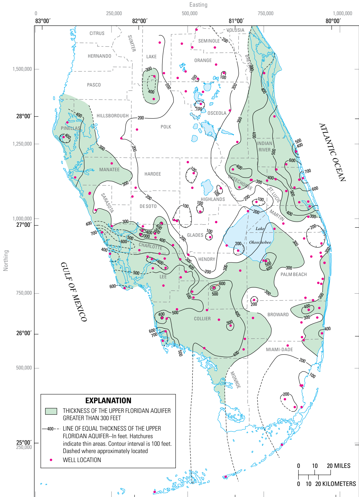
Figure 19. Thickness of the Upper Floridan aquifer.
