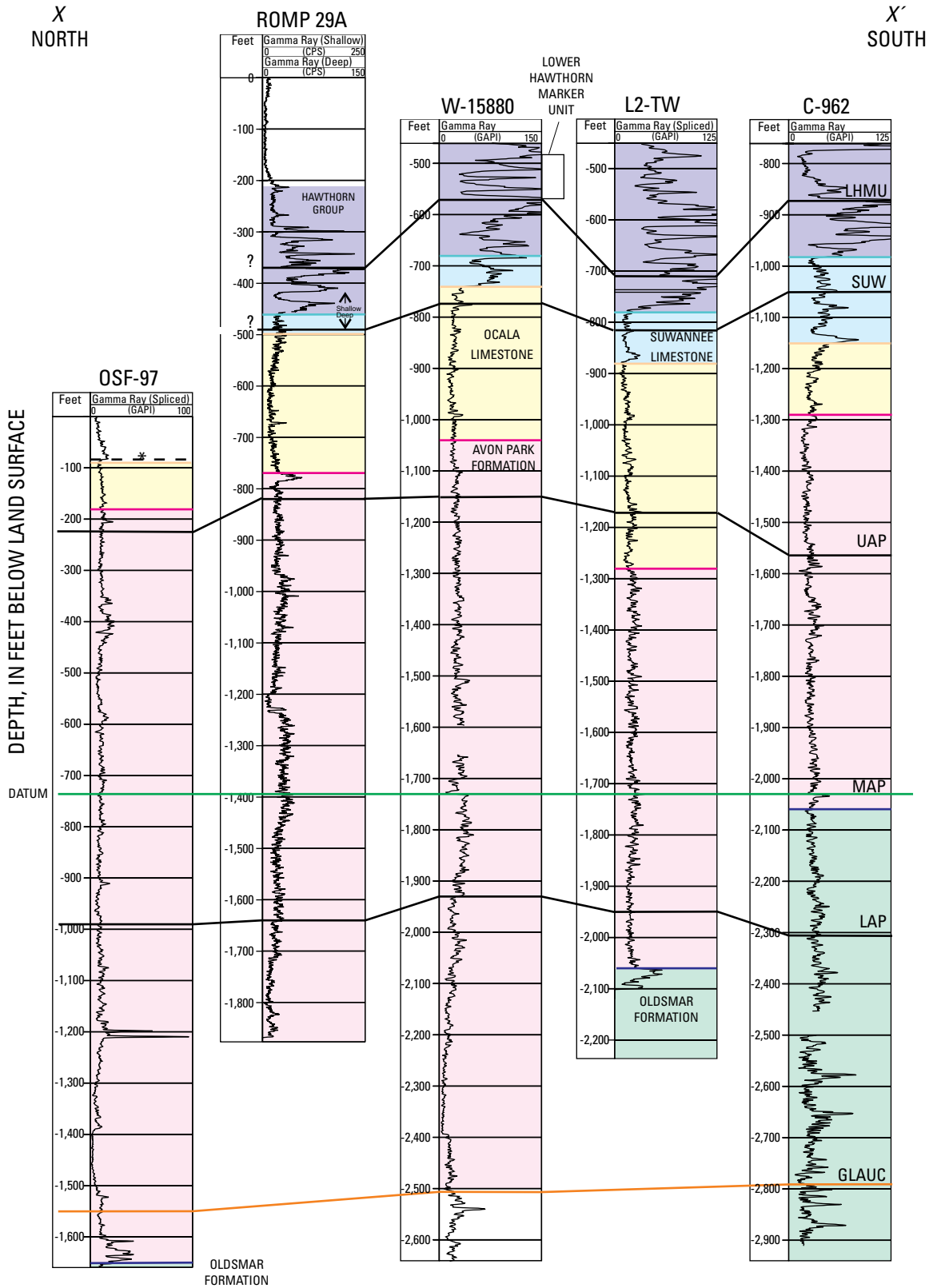
Figure 10c. Stratigraphic section X-X'. Trace of section shown in figure 9.
