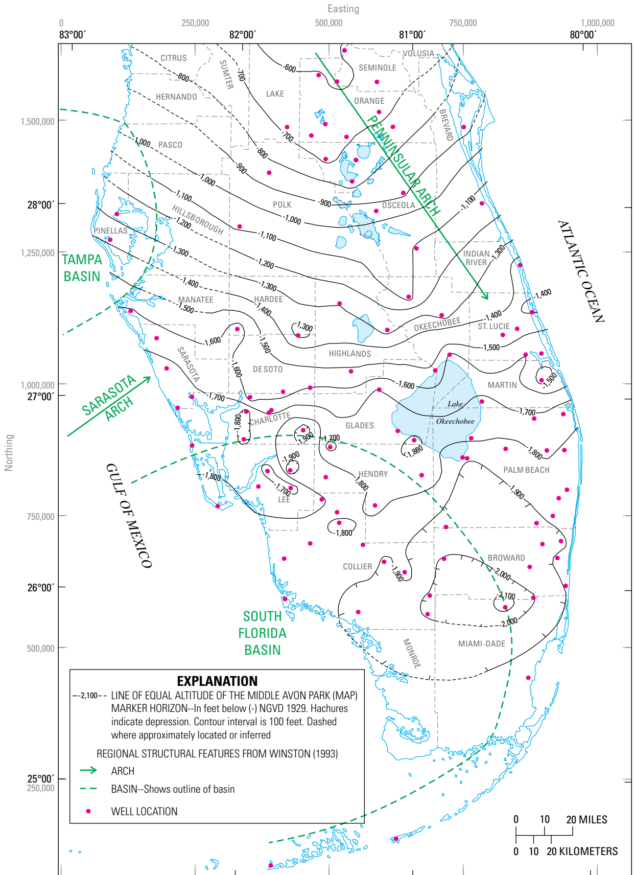
Figure 11. Altitude of the middle Avon Park marker horizon.
