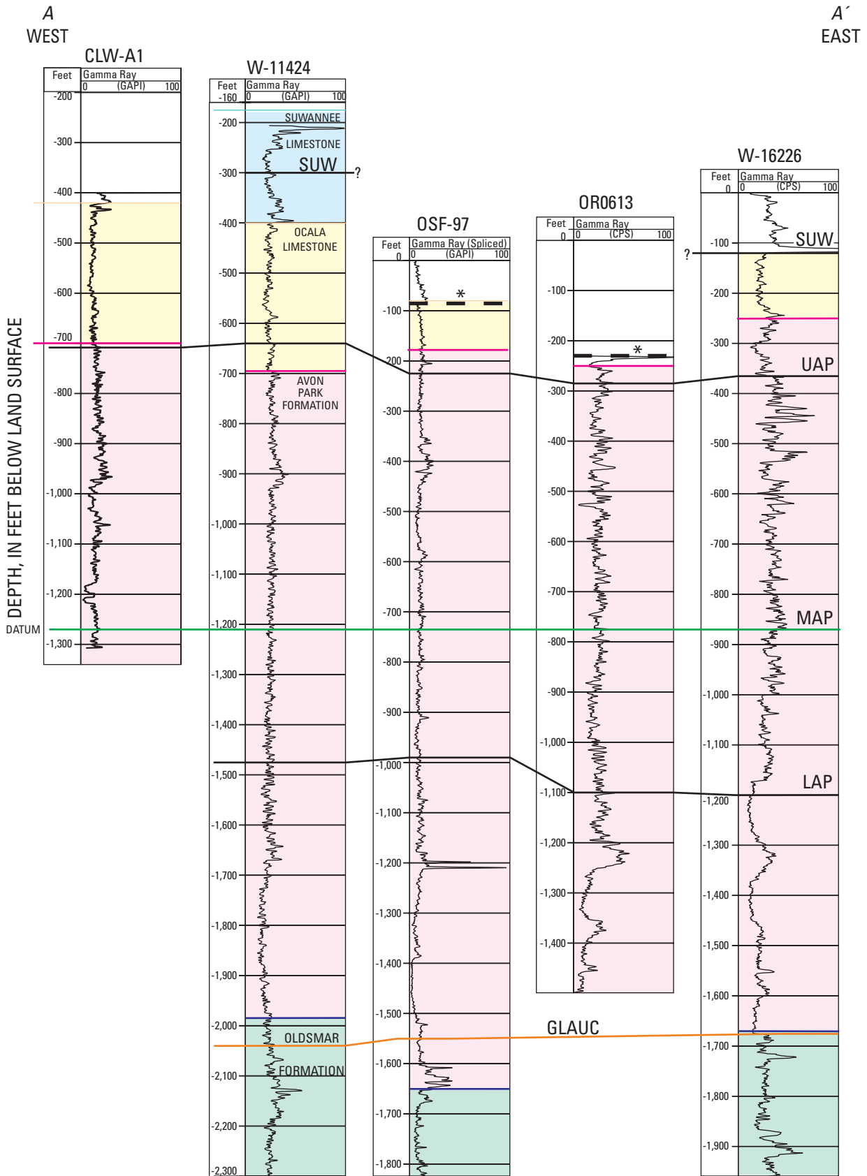
Figure 10a. Stratigraphic section A-A'. Trace of section shown in figure 9.
