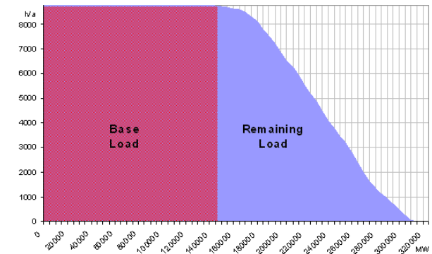
Fig. 3: Definition of base load and remaining load: full load hours in dependence on the demand power.
