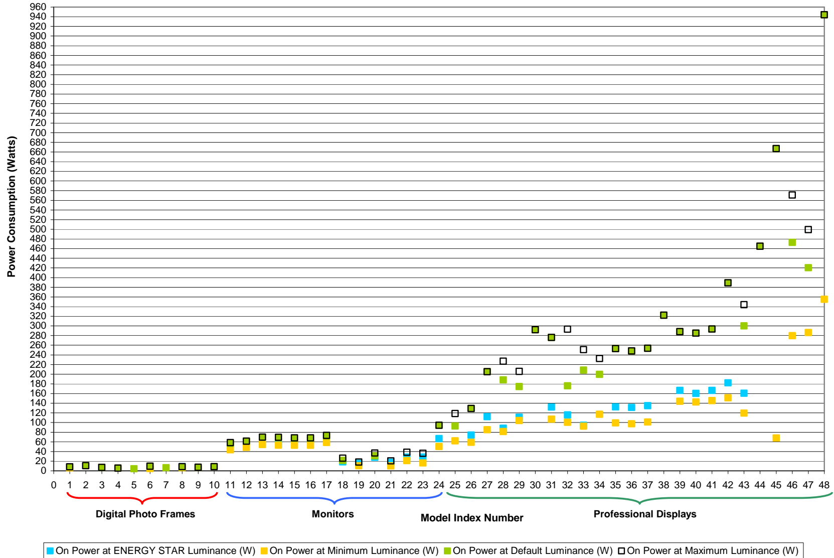
Chart showing On Mode Power Consumption at Minimum, Maximum, Default and ENERGY STAR Luminance Levels
