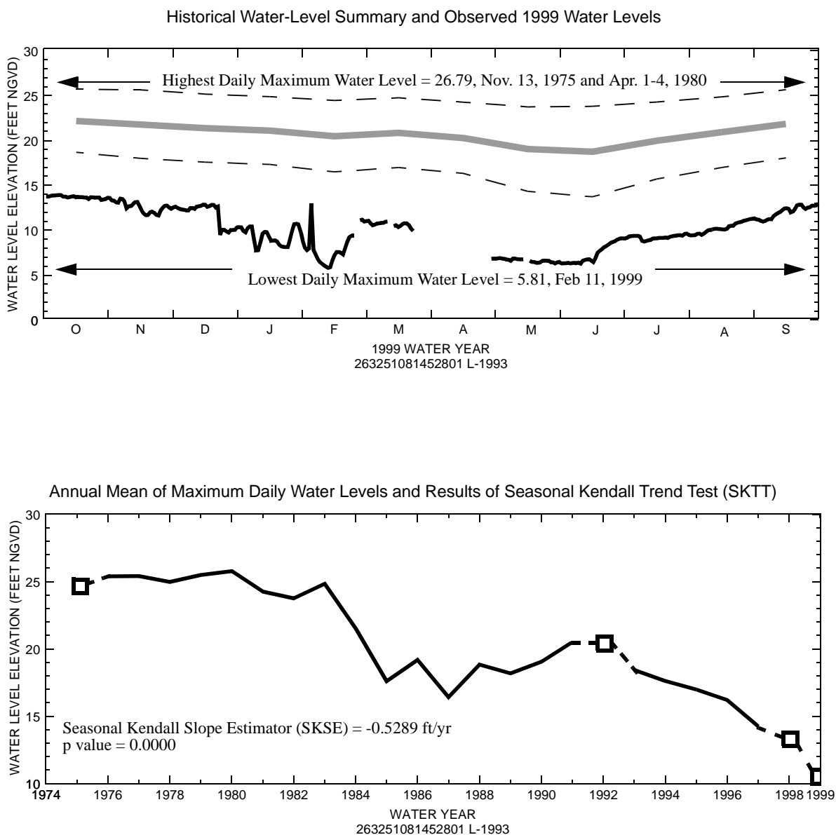
Figure 10. Historical water-level summary curves and annual mean of maximum daily water levels at well L-1993 penetrating the mid-Hawthorn aquifer. Explanation of plots is shown later in the Hydrologic Conditions.
