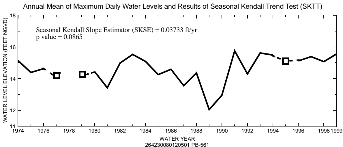
Figure 6. Historical water-level summary curves and annual mean of maximum daily water levels at well PB-561 penetrating the surficial aquifer system. Explanation of plots is shown later in the Hydrologic Conditions.
