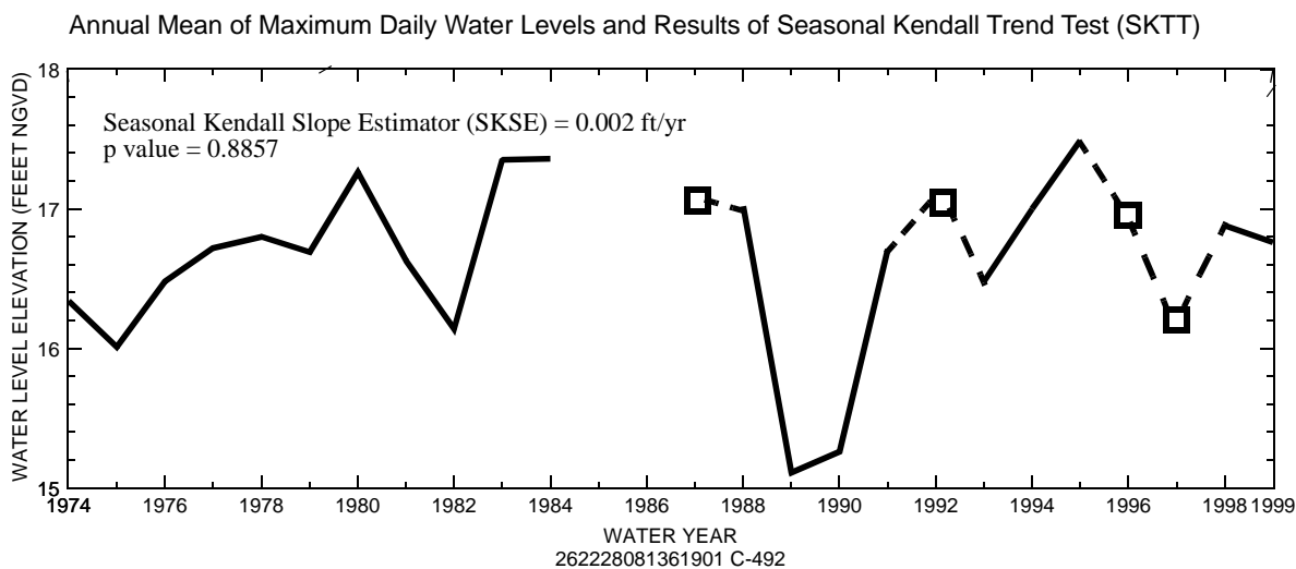
Figure 8. Historical water-level summary curves and annual mean of maximum daily water levels at well C-492 penetrating the Tamiami aquifer. Explanation of plots is shown later in the Hydrologic Conditions.
