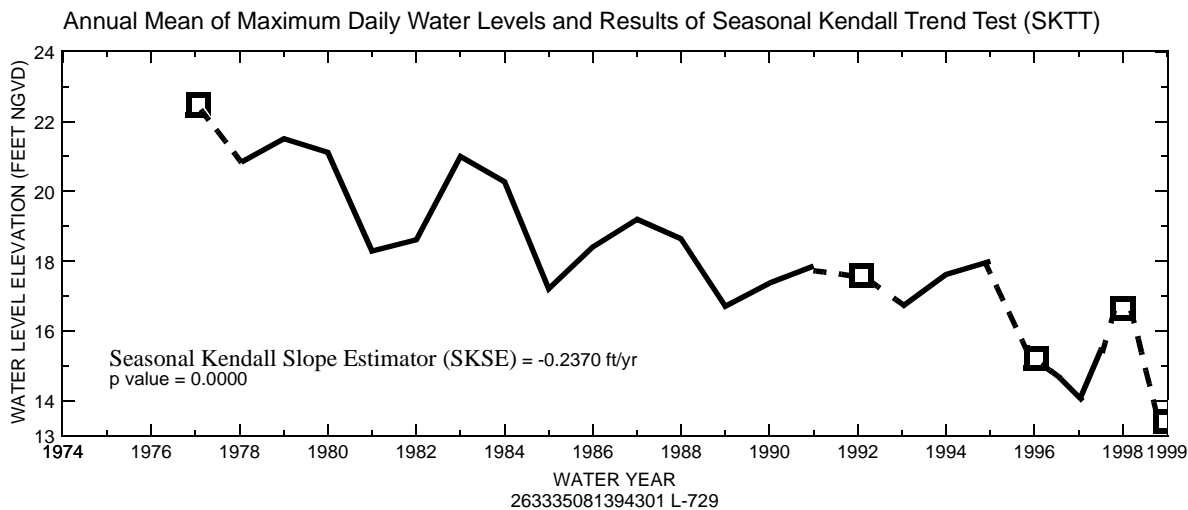
Figure 9. Historical water-level summary curves and annual mean of maximum daily water levels at well L-729 penetrating the sandstone aquifer. Explanation of plots is shown later in the Hydrologic Conditions.
