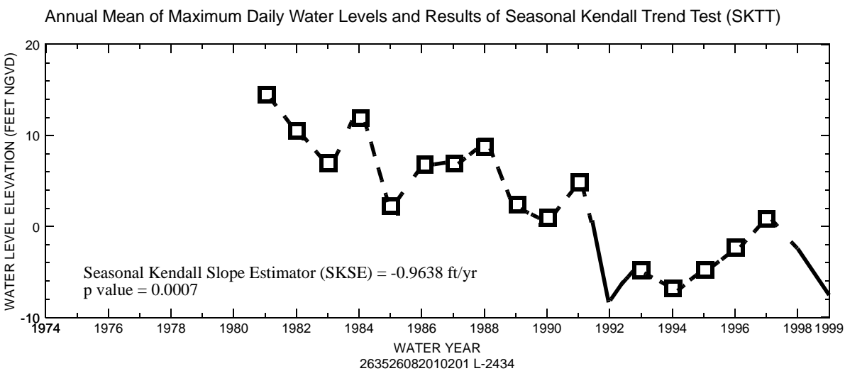
Figure 11. Historical water-level summary curves and annual mean of maximum daily water levels at well L-2434 penetrating the lower-Hawthorn producing zone. Explanation of plots is shown later in the Hydrologic Conditions.
