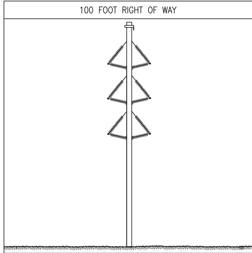
100 FOOT RIGHT OF WAY PROPOSED STEEL MONOPOLE 'HORIZONTAL VEE' 69-kV / 138-kV DOUBLE CIRCUIT
