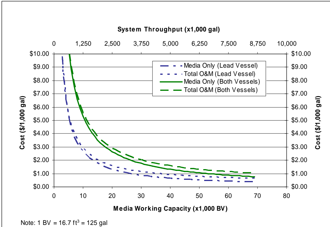
Figure 4-11. Media Replacement and O&M Cost without pH Adjustment
