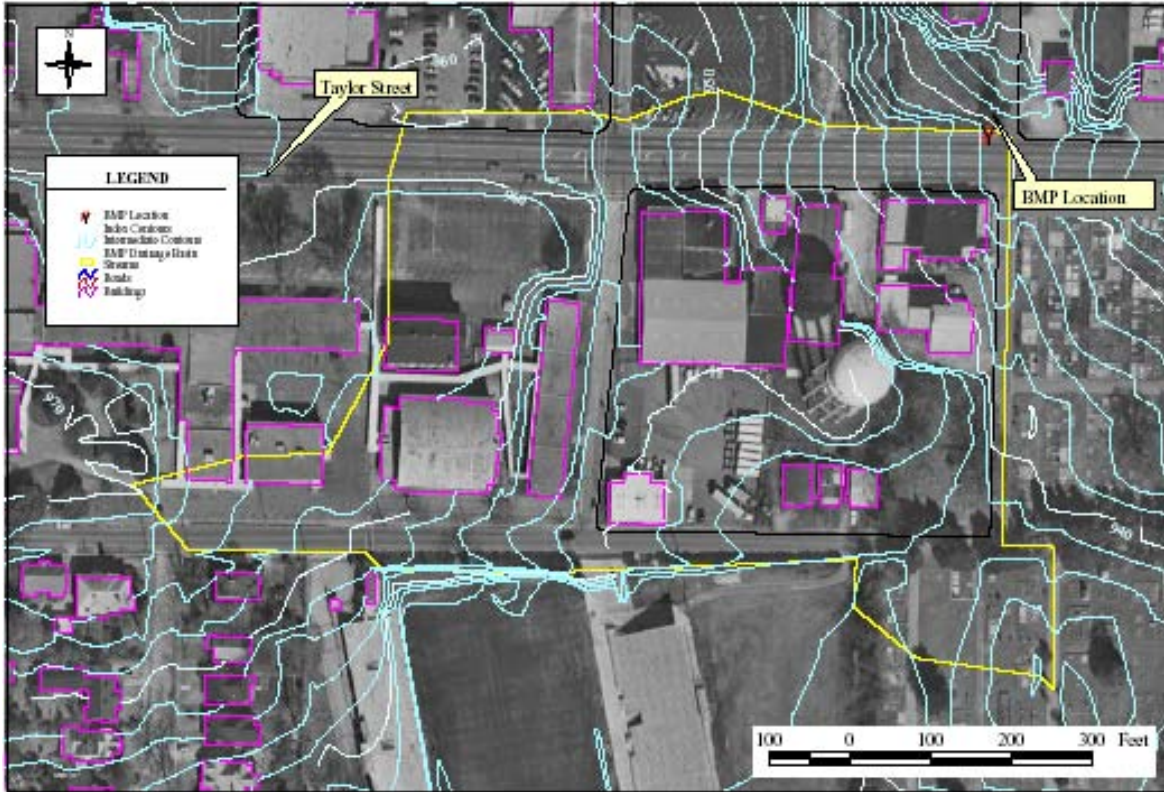
Figure 3-2. Drainage basin map for the BaySaver installation.
