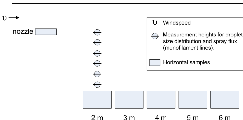
Figure 4. Low speed wind tunnel sampling locations.
